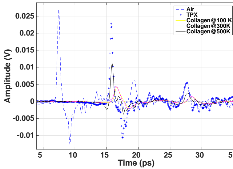
Fig. 4 THz transmission through reference plate TPX, air and cultured collagen samples of varying ( 1 \times 10^5 , 3 \times 10^5 and 5 \times 10^5 ) number of fibroblasts cells with stock solution concentration fixed.
