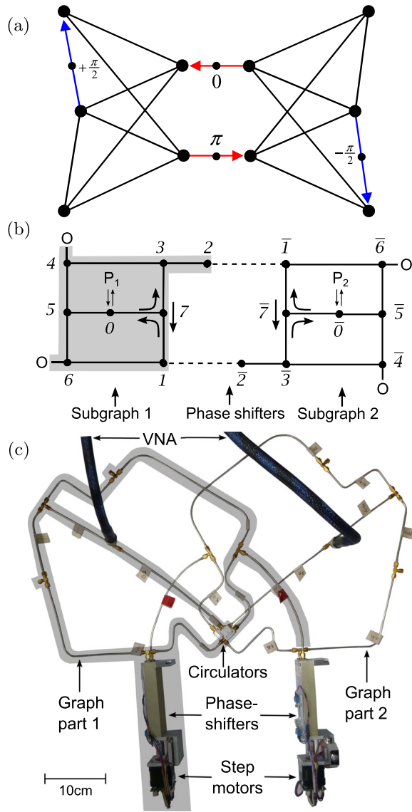
FIG. 1. (a) Sketch of the graph proposed in Ref. [21] to study GSE statistics without spin. The four arrows denote bonds along which additional phases are acquired. (b) Schematic drawing of one of the realized microwave graphs. Subgraph 1 is highlighted by a gray background. The dashed lines correspond to phase shifters with variable lengths. The two subgraphs contain microwave circulators at nodes 7 and \bar{7} , respectively, with opposite sense of rotation. The nodes marked by “O” are closed by open end terminators. They were used to allow for an easy realization of alternative graphs. Subgraphs 1 and 2 are connected at nodes 0 and \bar{0} , respectively, to ports P_1 ( P_2 ) of the VNA. (c) Photograph of the graph sketched in (b) consisting of T junctions, semirigid cables with identification tags, circulators, open end terminators, and phase shifters with step motors. Again, subgraph 1 is highlighted.
