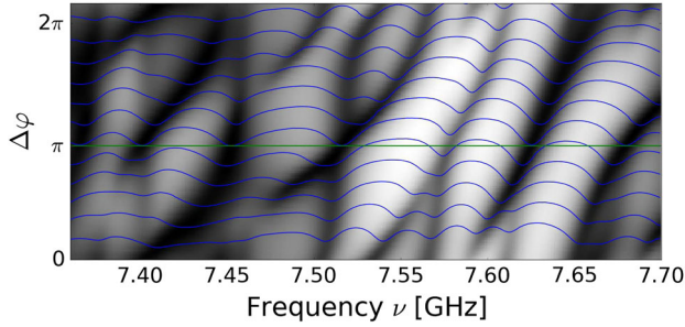
FIG. 3. Reflection |S_{11}|^2 in dependence of frequency in a shade plot. The results for different \Delta\varphi are stacked onto each other.
