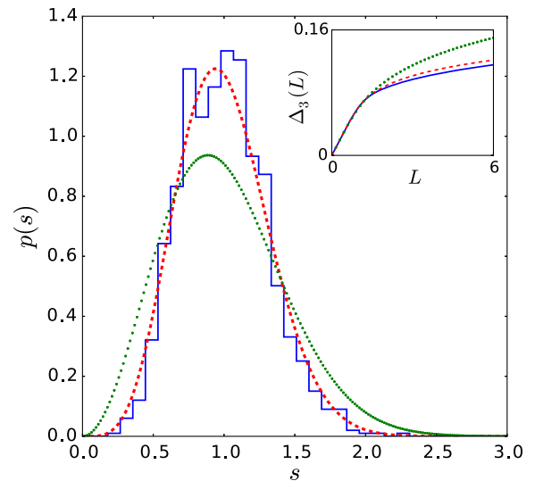
FIG. 4. Spectral nearest neighbor distance distribution obtained by superimposing the results from eight different spectra (blue). The dashed red and dotted green lines correspond to GSE and GUE Wigner distributions, respectively; see Eqs. (12) and (13). The inset shows the spectral rigidity for the same data set (blue), again with random matrix predictions for the GSE and the GUE in red and green, respectively.
