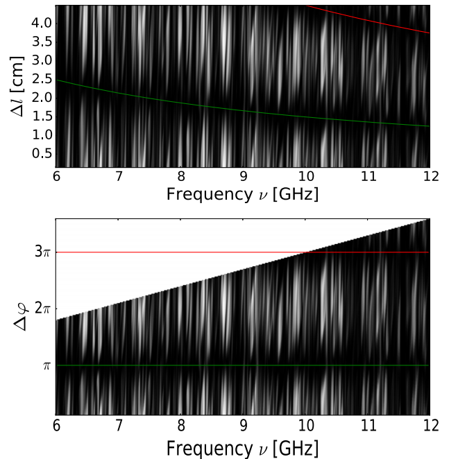
FIG. 2. (Top) Transmission |S_{12}|^2 in dependence of frequency for constant \Delta l in a gray scale, where black corresponds to zero and white to maximal transmission. The measurements for different \Delta l are stacked onto each other. (Bottom) The same data but rearranged to constant \Delta\varphi .
