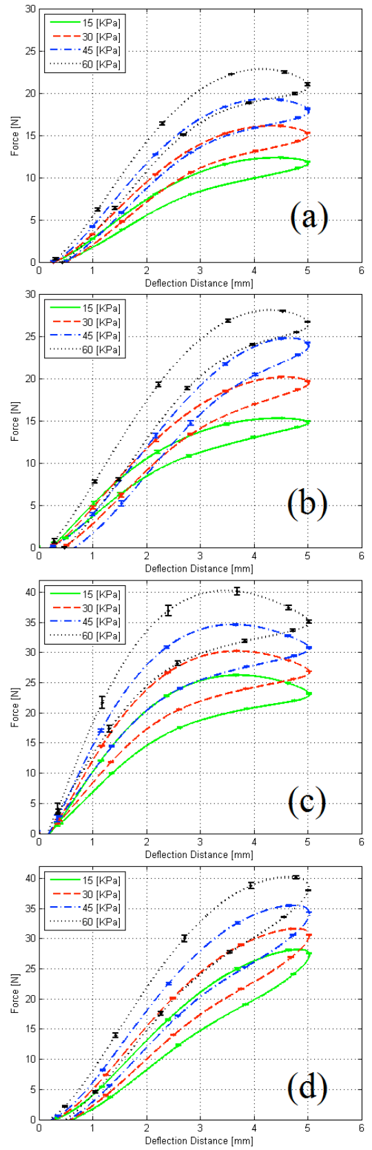
Figure 5: Deflection versus force at the link tip longitudinally applied for samples (a), (b), (c) and (d) at 15KPa, 30KPa, 45KPa and 60KPa. Standard deviation values ordered by increasing pressure level: (a) 0.051, 0.080, 0.089, 0.153; (b) 0.150, 0.136, 0.178, 0.179; (c) 0.133, 0.123, 0.206, 0.536; (d) 0.095, 0.100, 0.121, 0.255.
