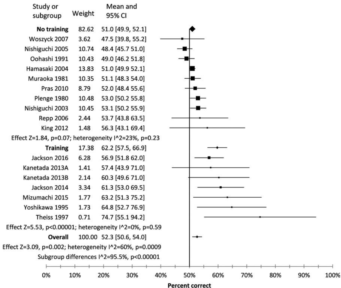
Fig. 2. A forest plot of studies where mean and standard deviation over all participants can be obtained, divided into subgroups based on whether participants were trained.
