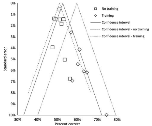
Fig. 3. Funnel plots of the 17 studies where a mean difference per participant was obtained, along with associated 95% confidence intervals. Much of the asymmetry in the overall funnel plot that might be attributed to publication bias is removed when funnel plots are given for subgroups of studies with and without training.
