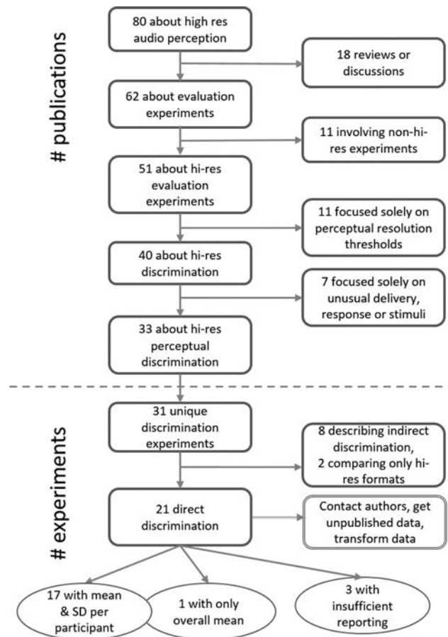
Fig. 1. Flowchart highlighting the study selection process.
