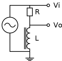
Figure 2: Passive high pass filter
