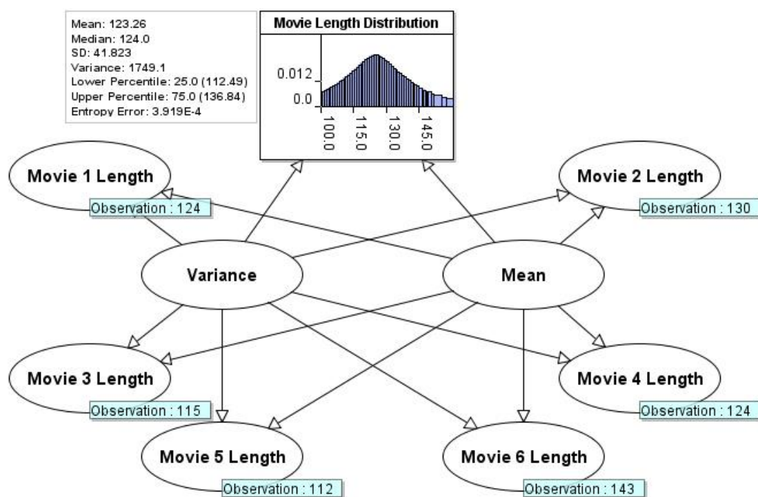
Figure 30: Induction Idiom Example
