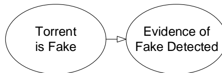
Figure 11: Basic BN for Fakes Detection
