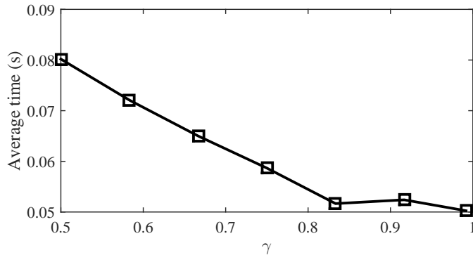
Figure 5: Average computational time versus \gamma = h_2/h_1 .
