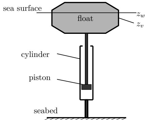
Figure 1: Schematic diagram of the point absorber
