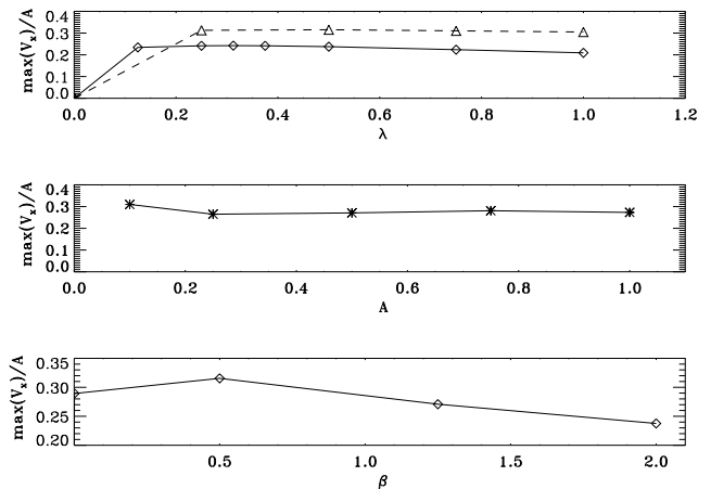
FIG. 4: Top panel: Maximal values of the relative amplitude of the generated compressible perturbations for different values of the inhomogeneity parameter \lambda , with \beta = 2 (solid curve) and \beta = 0.5 (dashed curve). The initial amplitude of the Alfvénic pulse is A = 0.5 . Mid panel: Maximal values of the relative amplitude of the generated compressible perturbations for different values of initial amplitude of the Alfvénic pulse, with inhomogeneity parameter \lambda = 0.5 and \beta = 1.25 . Bottom panel: Maximal values of the relative amplitude of the generated compressible perturbations for different values of \beta , with initial amplitude of the Alfvénic pulse A = 0.5 and inhomogeneity parameter \lambda = 0.5 .
