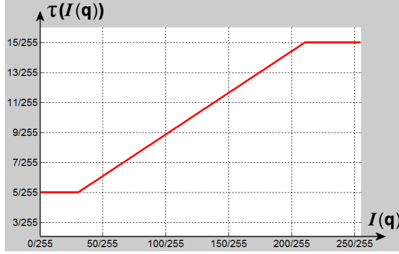
Fig. 6: Graphical representation of \tau(I(q)) .
