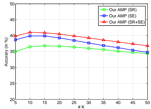
Figure 7. The performance (top-5 results in %) of our AMP methods with respect to different settings of the parameter K .
