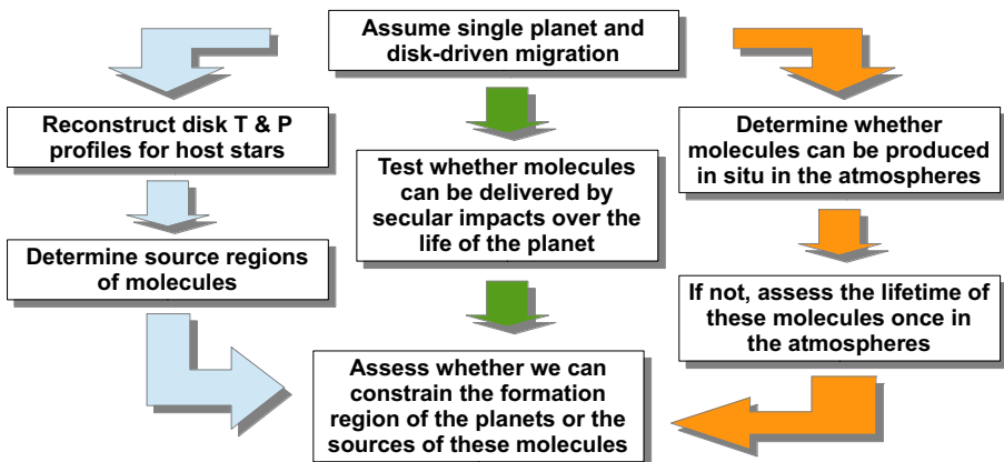
Fig. 8 A possible schematic approach to interpret the origins of molecular species in exoplanetary atmospheres
