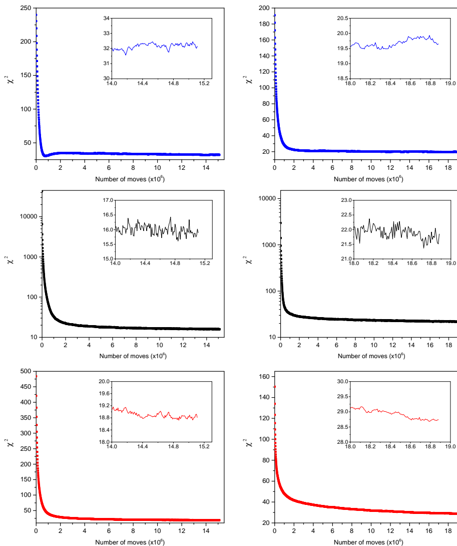
Figure S1: Representative \chi^2 plotted as a function of the number of atomic moves made for the Bragg I(t) (top), PDF D(r) (middle), and scattering function F(Q) (bottom) fits to 298 K (left) and 150 K (right) data.
