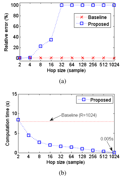
Fig. 13. (a) Distance estimation error and (b) computation time at different hop sizes by the baseline and the proposed methods. The inter-device distance is 4m . Two end-fire sources and two interferences. The signal length is 10s .
