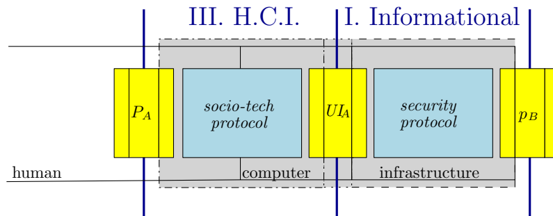
Fig. 2. The two-layered security ceremony instantiated over the infrastructure: the focus of example use 1 of our ceremony concertina traversal methodology is shaded
