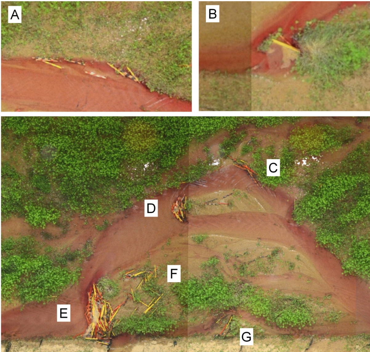
Figure 9: Comparisons between flume-scale and field-scale wood deposition patterns: single-thread / wandering morphology
