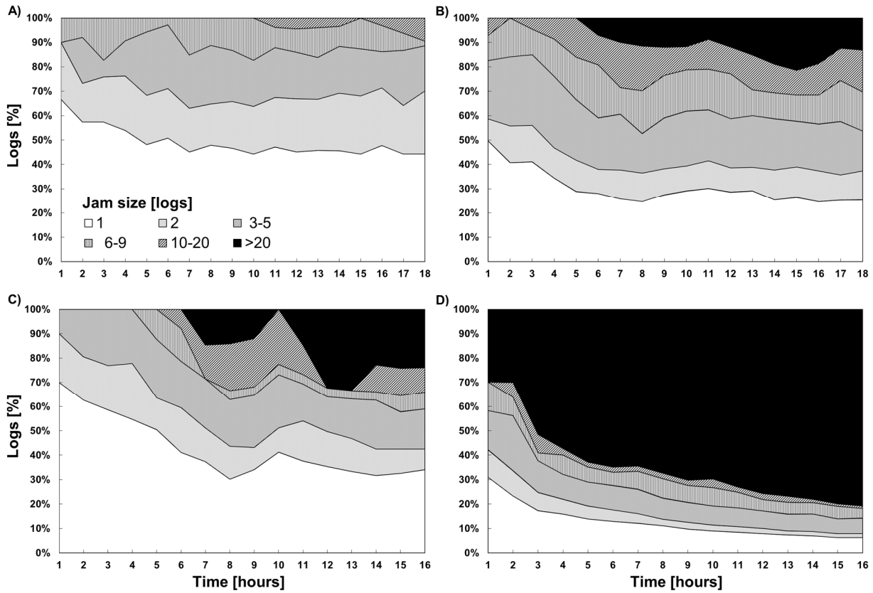
Figure 5: The proportion of logs stored in jams of different size under A. unvegetated, low wood input regime; B. unvegetated, high wood input regime; C. vegetated, low wood input regime; D. vegetated, high wood input regime.
