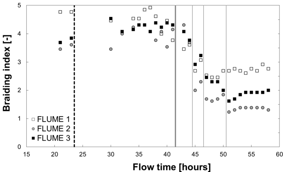
Figure 3: Changes in the reach-averaged braiding index during high flows through the sequence of experiments (the dashed vertical line marks the commencement of the wood experiments, the solid vertical grey line marks the commencement of the vegetation experiments at the first cycle (which includes the one hour high flow preparation of the flumes prior to commencement of log introduction for 2 hours), followed by three thin grey lines marking the ends of the second, third and fourth high flow cycles under vegetated conditions).
