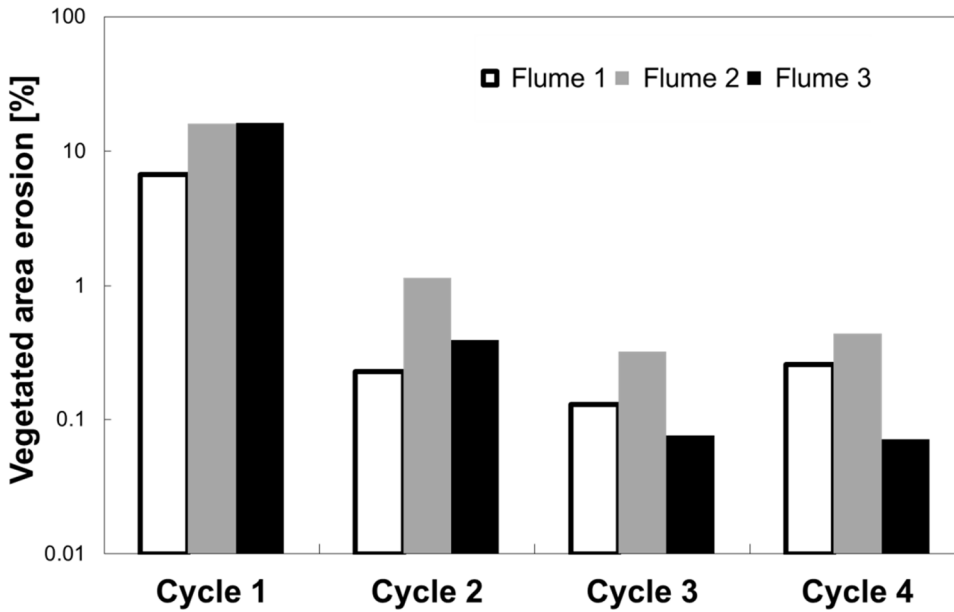
Figure 2. The proportion of the vegetated area eroded within the three flumes during each of the four cycles.
