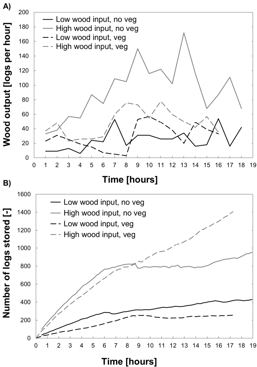
Figure 4 Wood retention and delivery from the flume during 18 hours of high flows under low and high wood input regimes and with no vegetation and a vegetation cover present. A. The number of logs output from the flume each hour. B. The number of logs retained within the flume at the end of each hour.
