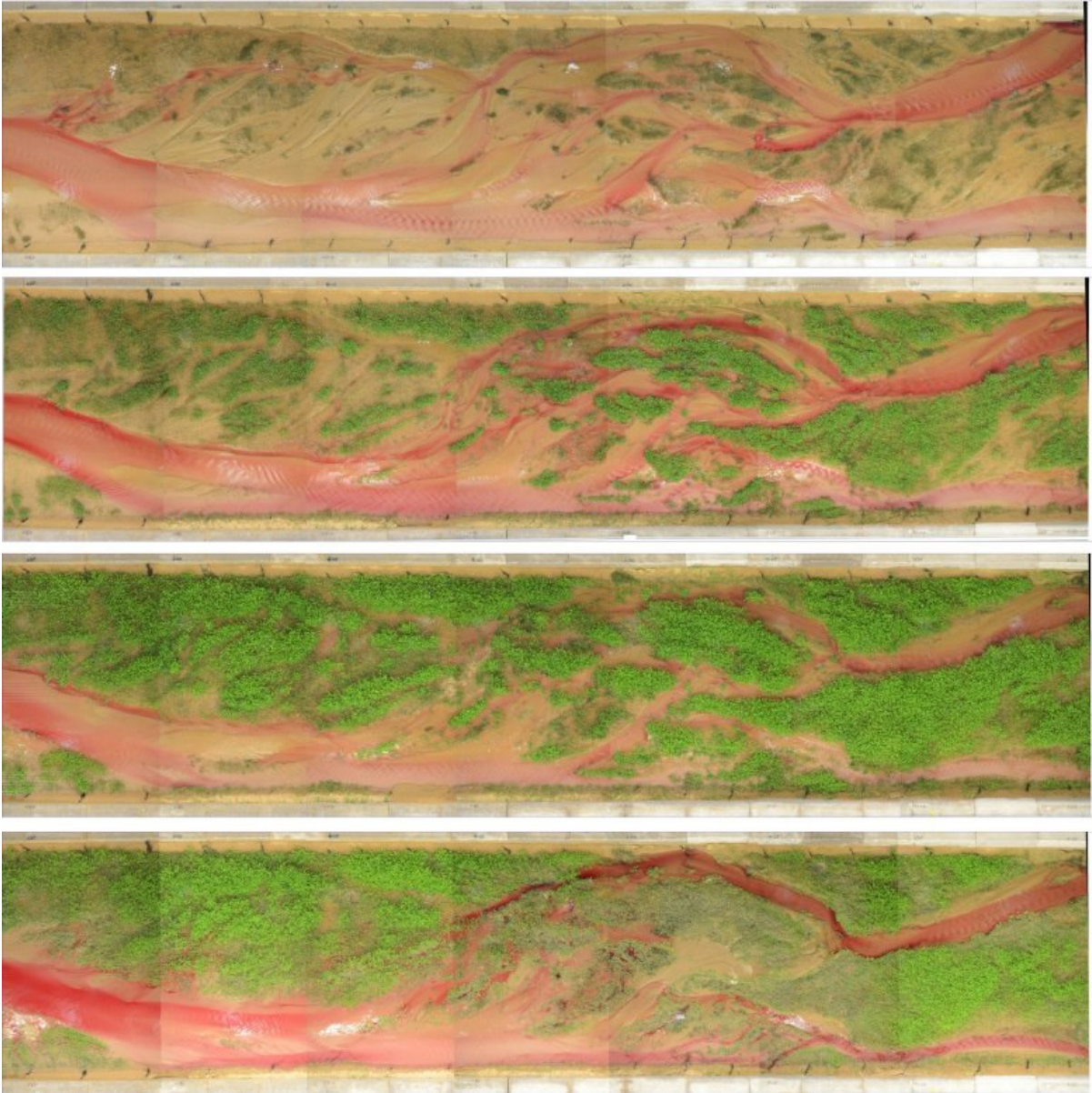
Figure 1. Vegetation distribution in flume 1 (no wood) at the end of each of the four high flow cycles illustrated in chronological order from top to bottom.
