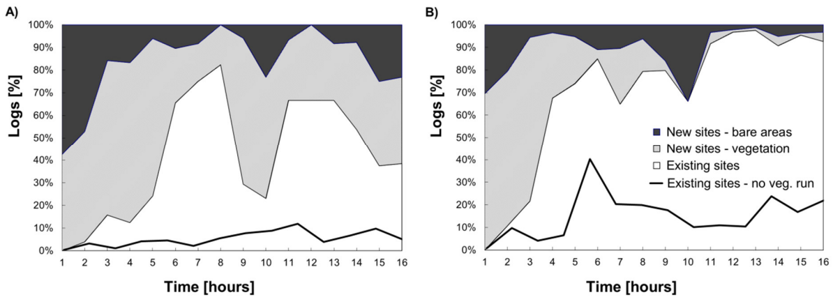
Figure 7. The proportion of new logs deposited within vegetated flumes on bare sediment (dark grey), vegetation (light grey), and previously deposited logs (white) under A. a low wood input regime and B. a high wood input regime. The heavy black line refers to new logs deposited on previously deposited wood in unvegetated flumes under the same wood input regime.
