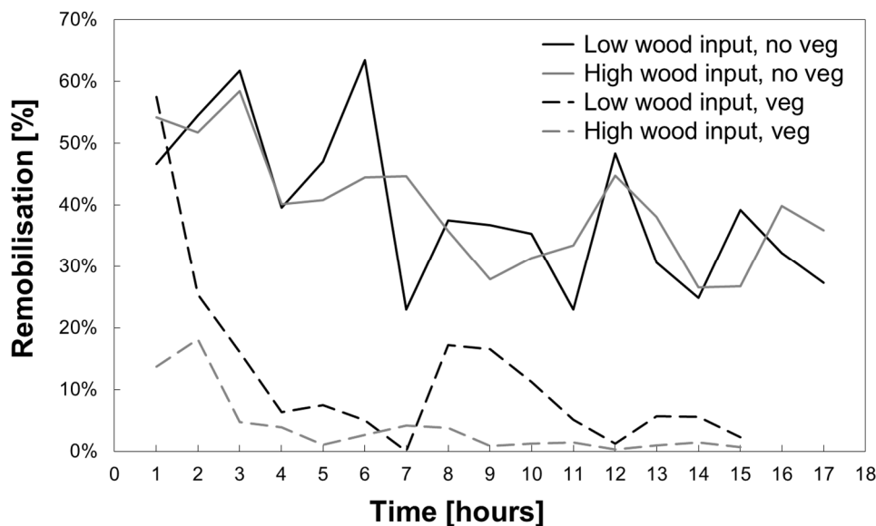
Figure 6. Log remobilisation under the presence and absence of vegetation and low and high wood input regimes (wood remobilisation is computed as the ratio of the number of logs delivered from the flume during each hour as a proportion of the number of logs stored within the flume at the beginning of each hour)
