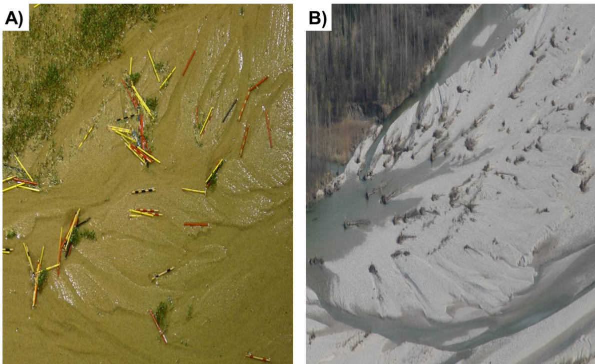
Figure 8: Comparisons between flume-scale and field-scale wood deposition patterns: braided morphology
