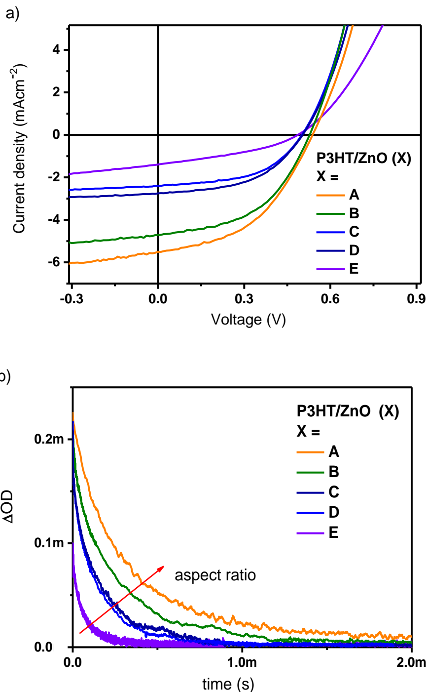
Figure 2 J-V curves (a) and transient absorption signals (b) of P3HT/ZnO(X) active layers with aspect ratios of A:38, B:30, C:20, D:19, E:5. Transient absorption data measured under N 2 atmosphere, probed at 980 nm and excited at 500 nm with an excitation intensity of 6 μJcm -2 . The y-axis (ΔOD) corresponds to charge photogeneration yield.
