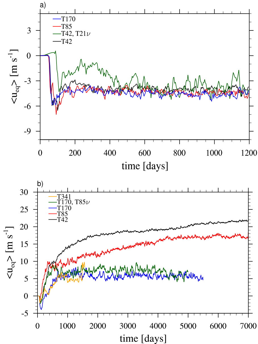
Figure 5.13: Time series of column-averaged zonal wind at the equator \langle u_{\text{eq}} \rangle [m s -1 ] at varying horizontal resolutions for the control simulations (a) and the RTG simulations (b): \langle u_{\text{eq}} \rangle for {T42L30, T85L30, T170L30, T341L30} resolutions are shown in {black, red, blue, yellow}, respectively. The green curve in a) shows the control simulation performed at T42 horizontal resolution with \nu_8 from a T21 resolution simulation, which is 25 times larger than in the “nominal” T42 simulation (black curve). The green curve in b) shows the RTG simulation performed at T170 horizontal resolution with \nu_8 same as in the T85 resolution simulation (red curve). The magnitude of \langle u_{\text{eq}} \rangle is insensitive to horizontal resolution in the control simulations – when properly tuned , whereas \langle u_{\text{eq}} \rangle decreases with increasing resolution in the RTG simulations. In the latter simulations, T170L30 simulations with different \nu_8 produce nearly-identical results.
