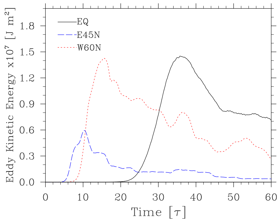
Figure 3.7: Evolution of globally-averaged eddy kinetic energy (per area) [ \text{J m}^{-2} ] for runs E45N (dashed blue line), W60N (dotted red line) and EEQ (solid black line). The eddy kinetic energy for EEQ has been multiplied by a factor of 40.
