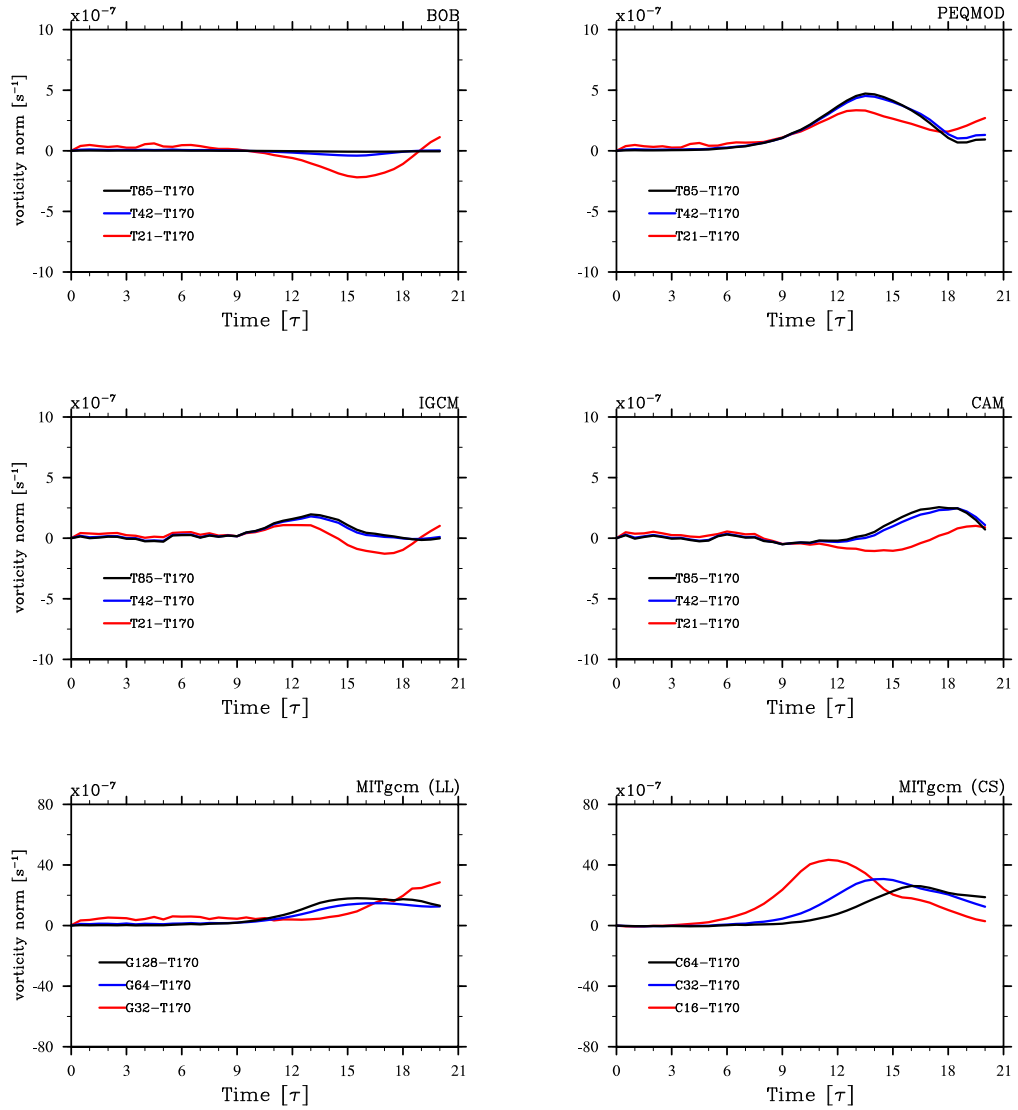
Figure 4.8: Differences of the root mean square l_2 vorticity norm [ s^{-1} ] between T170L20 reference solution for BOB and solutions with other dynamical cores at various resolutions. The scales are same as in Figure 4.7. The T42 simulations in all the pseudospectral cores appears to be marginally “intra-converged”. MITgcm core in both LL and CS grids are not converged, particularly in the latter grid.
