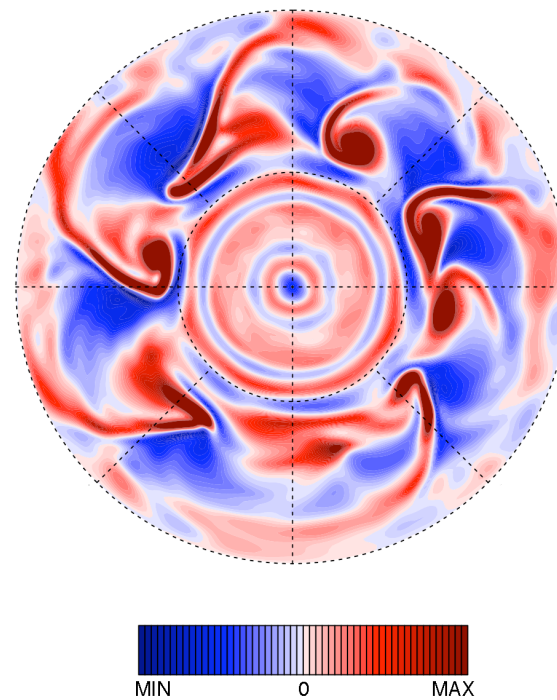
Figure 3.16: Temperature T (top) and relative vorticity \zeta (bottom) for run EEQ in polar stereographic view, centred on the north pole. The fields are shown at 975 hPa pressure level for t = 26 \tau . Maximum and minimum values for temperature are 1460 K and 1600 K, respectively, with contour interval 3.5 K. Values for \zeta are in the range \pm 1.5 \times 10^{-5} \text{s}^{-1} , with contour interval 6 \times 10^{-7} \text{s}^{-1} .
