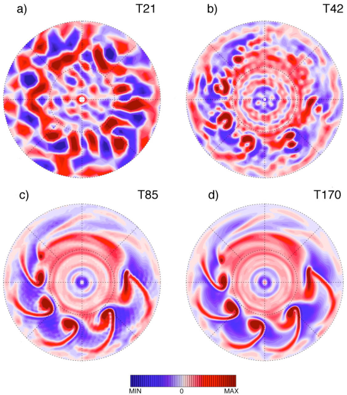
Figure 3.17: Polar stereographic view of the relative vorticity field \zeta , centred on the north pole, for four runs with all parameters identical – except the horizontal resolution. The common parameters are as in run EEQ. The fields at t = 22 \tau are shown. The number at upper right in each panel indicates the resolution. Contour levels are the same to those in Figure 3.16.
