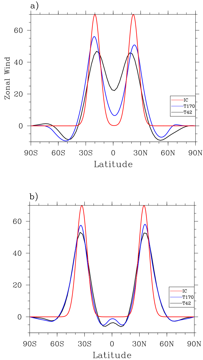
Figure 5.10: Initial zonal wind u_0(\phi) [ \text{m s}^{-1} ] (red curve) and equilibrated zonal-mean zonal wind ( \bar{u} ) [ \text{m s}^{-1} ] at T170 (blue curve) and T42 (black curve) horizontal resolutions from initial value calculations with the shallow-water model. In a ) u_0 satisfies the necessary condition for barotropic instability at \phi \sim \pm 5^\circ . In b ) u_0 satisfies the necessary condition for barotropic instability – but further from the equator than in a ). In a ) superrotation is produced as a result of mixing at the equator whereas in b ) mixing is located further away from the equator and superrotation is not produced. Note also stronger superrotation in T42 simulation in a ).
