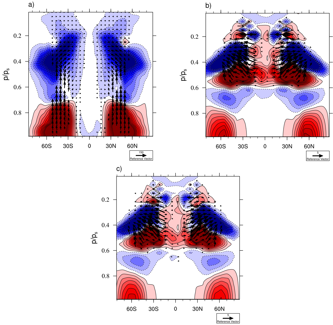
Figure 5.5: Eliassen-Palm flux vector, \mathbf{F} = (F_\phi, F_p) [ \text{m}^2 \text{s}^{-2} ], and its divergence, \mathcal{E} = \nabla \cdot \mathbf{F} [ \text{m s}^{-2} ], fields for the control simulation (a) and the RTG simulation (b and c) at T170L30 resolution. a): time-average during a statistically steady state, over t = [700, 1200] days. b) and c): RTG simulation time-average during the acceleration stage, over t = [200, 700] days and during a statistically steady state, over t = [4500, 5000] days, respectively. Negative \mathcal{E} values are dashed (and in blue) and positive values are solid (and in red). Maximum and minimum \mathcal{E} values are \pm 700 \text{ m s}^{-2} in (a) and \pm 100 \text{ m s}^{-2} in (b and c). The reference vector in (a) has magnitude of 150 \text{ m}^2 \text{s}^{-2} and in (b) and (c) of 5 \text{ m}^2 \text{s}^{-2} . F_\phi and F_p are scaled by 1 radian of latitude and 1 Pa of pressure, respectively. In addition, F_p is scaled by a factor of 0.5 in (b) and (c). The wave propagation is upward and equatorward in the control simulation, and upward and mainly poleward in the RTG simulation. The wave activity is changed little between the acceleration and the equilibrated stages in the RTG simulation: the largest differences occur at p \approx 500 \text{ hPa} level in the equatorial region, where the zonal flow acceleration is stronger during the acceleration stage.
