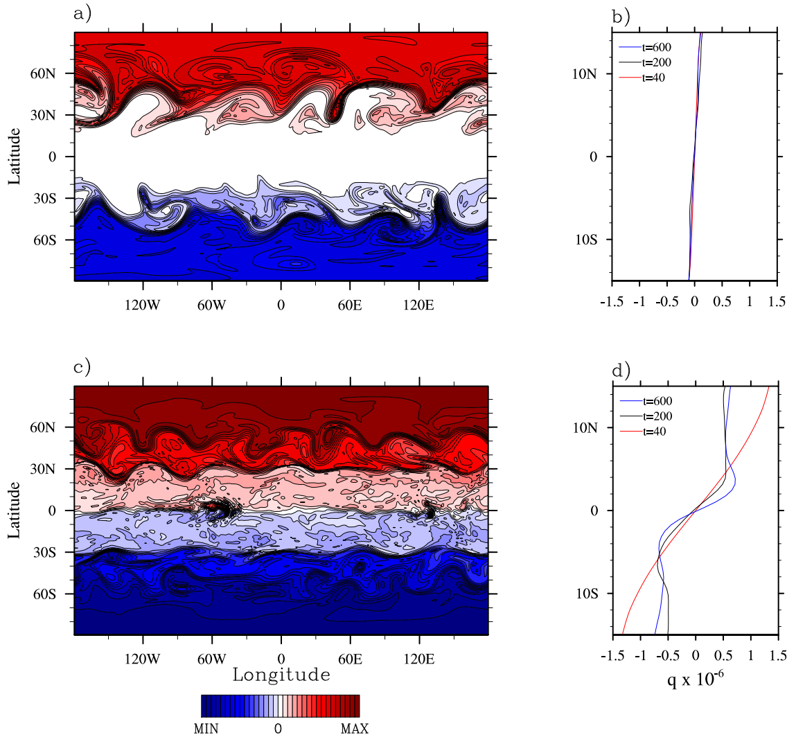
Figure 5.7: Snapshot of Ertel potential vorticity q [ \text{K m}^2 \text{kg}^{-1} \text{s}^{-1} ] and its zonal-mean \bar{q} for the control simulation ( a and b , respectively) and RTG simulation ( c and d , respectively) at T170L30 resolution. The q fields are shown at t = 600 days in cylindrical-equidistant projection on the \Theta = 315 \text{ K} and \Theta = 300 \text{ K} isentropes, respectively (these surfaces lie approximately at p = 500 \text{ hPa} in the tropics). Maximum and minimum contour values are \pm 10^{-5} \text{ K m}^2 \text{kg}^{-1} \text{s}^{-1} and \pm 5 \times 10^{-6} \text{ K m}^2 \text{kg}^{-1} \text{s}^{-1} , respectively. The m \sim 6 mode can be seen in both a ) and c ), as well as the presence of equatorial q -gradients and blobs in c ) (only). Panels b ) and d ) show \bar{q} on same isentropes as in a ) and c ). The equatorial region at t = 40 days (red), t = 200 days (black) and t = 600 days (blue) is shown. Superrotation is generated in the RTG simulation as a consequence of extrusion of high q from higher latitudes to the equator via mixing. In contrast, notice the absence of q -mixing at the equator in the control simulation.
