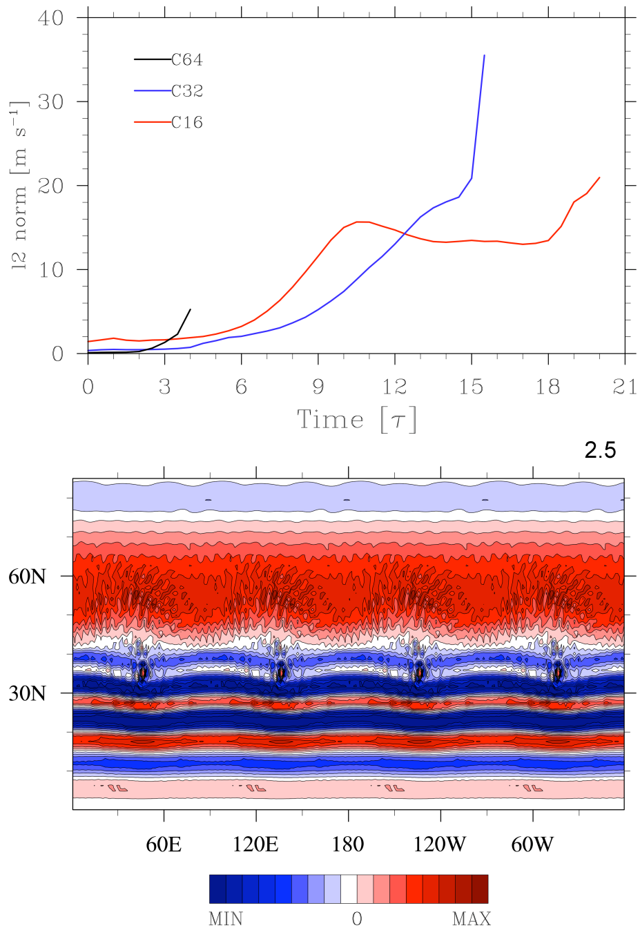
Figure 4.3: Top: Symmetry deviation l_2 -norm of [u(t) - \bar{u}(t)] [ \text{m s}^{-1} ] for MITgcm cubed-sphere (CS) steady-state case simulations in the default configuration. Three different resolutions (C16, C32, C64) are presented. Higher resolution simulation norms blow-up earlier. Bottom: \zeta field at t = 2.5 \tau , at the 975 hPa level, from the C64 resolution simulation in the top panel. Maximum and minimum values are +6 \times 10^{-7} \text{ s}^{-1} and -6 \times 10^{-7} \text{ s}^{-1} , respectively, with contour interval of 8 \times 10^{-8} \text{ s}^{-1} . The increase in the l_2 -norms in the top panel are caused by the special corner points, seen in the bottom panel. Note, the norms are not exactly zero initially, especially at low resolution. This is due to the errors introduced by the re-gridding procedure of u from LL to CS grid.
