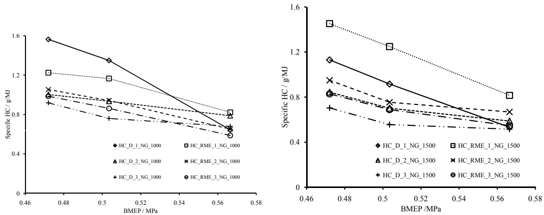
(a) Specific HC for natural gas combustion with three different diesel pilot and RME pilot fuel settings at 1000 rev/min (b) Specific HC for natural gas combustion with three different diesel pilot and RME pilot fuel settings at 1500 rev/min
