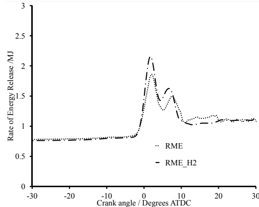
(b) Rate of energy release for pure RME and RME piloted hydrogen at a BMEP of 0.503 MPa and 1000 rev/min
