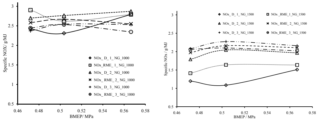
(a) Specific \text{NO}_X for natural gas combustion with three different diesel pilot and RME pilot fuel settings at 1000 rev/min (b) Specific \text{NO}_X for natural gas combustion with three different diesel pilot and RME pilot settings at 1500 rev/min
