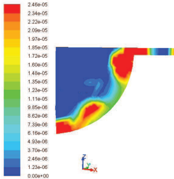
Figure 7.27. Contours of NO at 2^\circ ATDC using KHRT breakup model ( C_3 = 30 ) and unsteady flamlet approach
