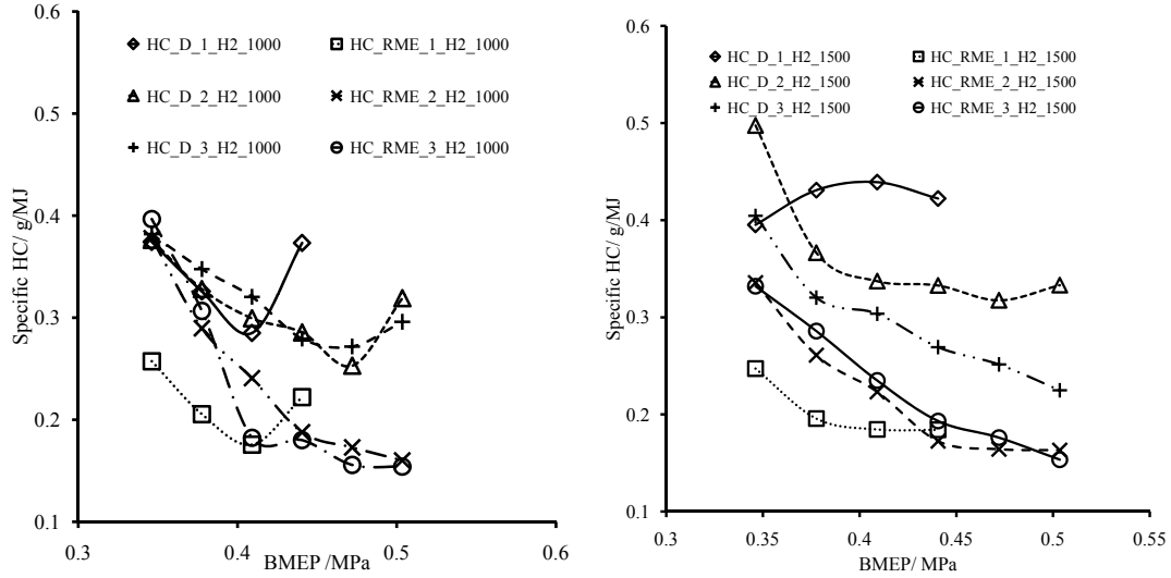
(a) Specific HC for hydrogen combustion with three different diesel pilot and RME pilot fuel settings at 1000 rev/min (b) Specific HC for hydrogen combustion with three different diesel pilot and RME pilot settings at 1500 rev/min
