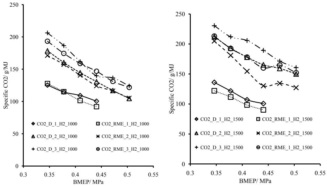
(a) Specific CO 2 for hydrogen combustion with three different diesel pilot and RME pilot fuel settings at 1000 rev/min (b) Specific CO 2 for hydrogen combustion with three different diesel pilot and RME pilot settings at 1500 rev/min
