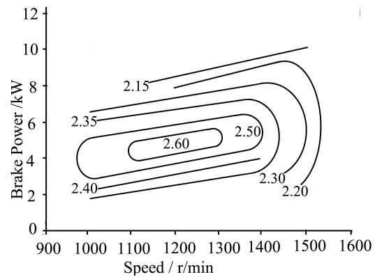
(b) Specific \text{NO}_X / g/MJ - RME
