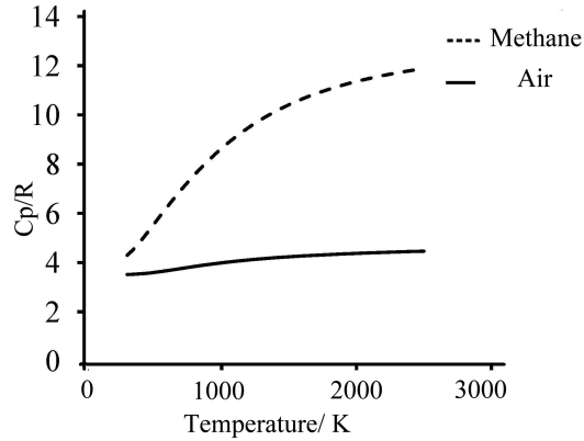
Figure 4.3. Specific heat at constant pressure, C_P/R as a function of temperature for air and methane
