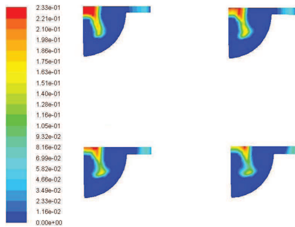
Figure 7.18. Contours of O_2 from 11^\circ ATDC to 14^\circ ATDC using KHRT breakup model ( C_3 = 30 ) and unsteady flamlet approach
