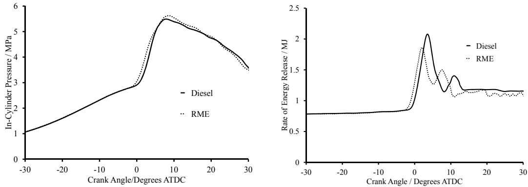
(a) Cylinder pressure for pure diesel and RME at a BMEP of 0.503 MPa and 1000 rev/min (b) Rate of energy release for pure diesel and RME at a BMEP of 0.503 MPa and 1000 rev/min
