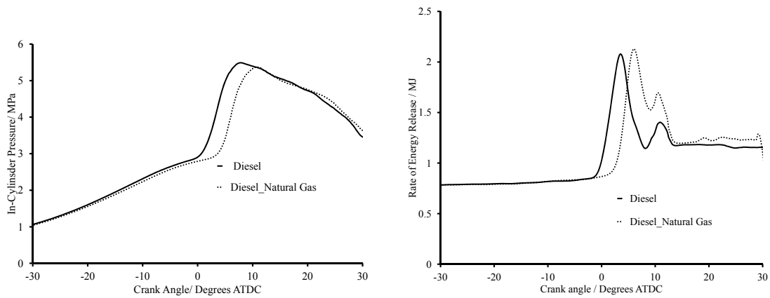
(a) Cylinder pressure for pure diesel and diesel piloted natural at a BMEP of 0.503 MPa and 1000 rev/min (b) Rate of energy release for pure diesel and diesel piloted natural gas at a BMEP of 0.503 MPa and 1000 rev/min
