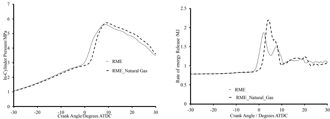
(a) Cylinder pressure for pure RME and RME piloted natural at a BMEP of 0.503 MPa and 1000 rev/min (b) Rate of energy release for pure RME and RME piloted natural at a BMEP of 0.503 MPa and 1000 rev/min
