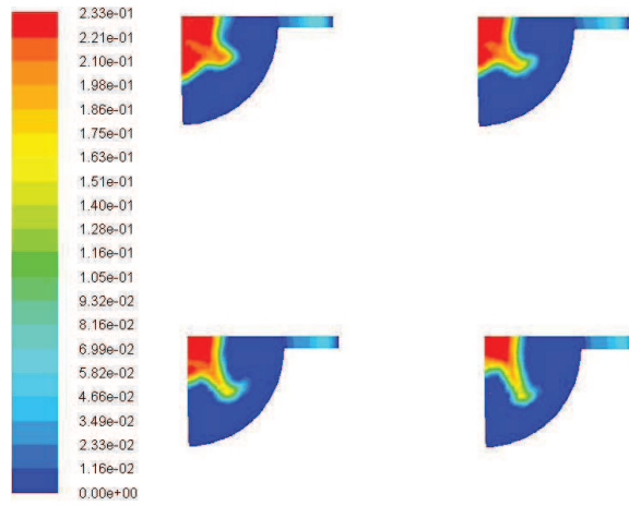
Figure 7.17. Contours of O_2 from 7^\circ ATDC to 10^\circ ATDC using KHRT breakup model ( C_3 = 30 ) and unsteady flamlet approach
