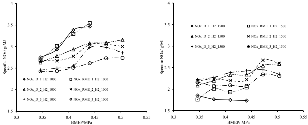
(a) Specific \text{NO}_X for hydrogen combustion with three different diesel pilot and RME pi- lot fuel settings at 1000 rev/min (b) Specific \text{NO}_X for hydrogen combustion with three different diesel pilot and RME pi- lot settings at 1500 rev/min
