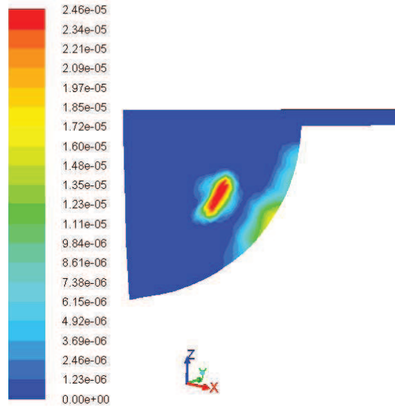
Figure 7.26. Contours of NO at -2^\circ ATDC using KHRT breakup model ( C_3 = 30 ) and unsteady flamlet approach
