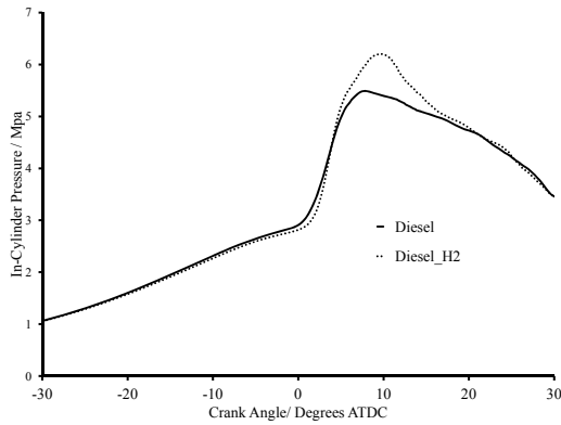
(a) Cylinder pressure for pure diesel and diesel piloted hydrogen at a BMEP of 0.503 MPa and 1000 rev/min
