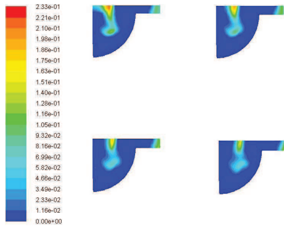
Figure 7.19. Contours of O 2 from 15° ATDC to 18° ATDC using KHRT breakup model ( C_3 = 30 ) and unsteady flamlet approach
