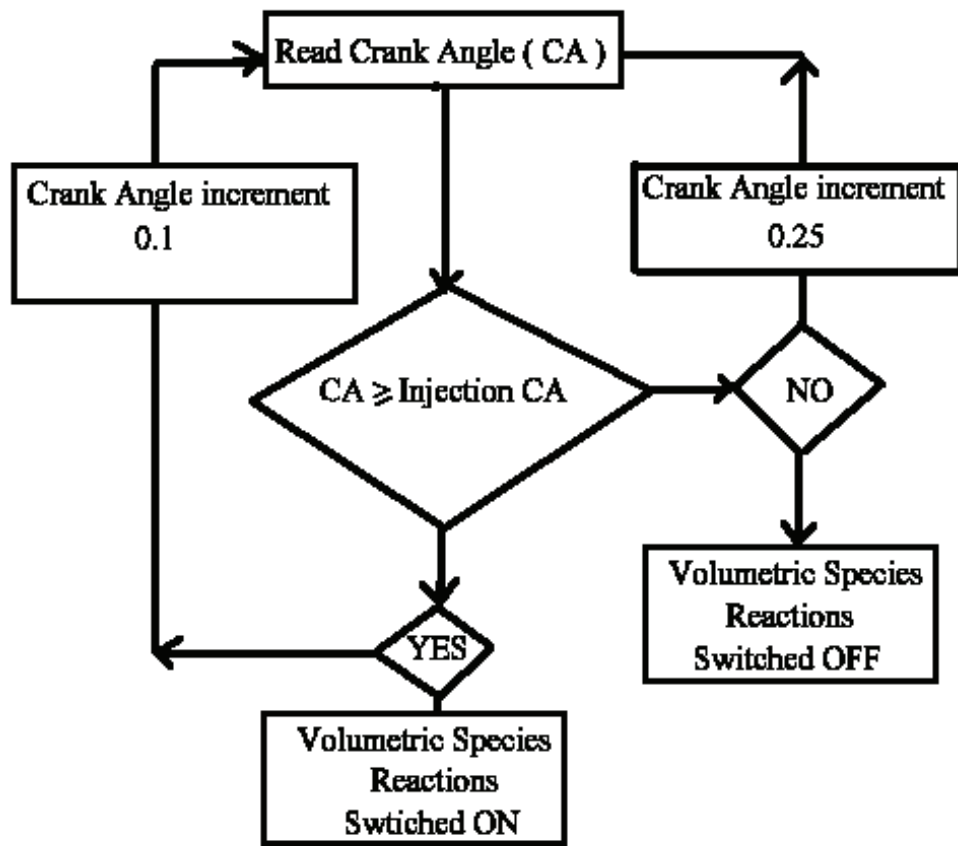
Figure 7.3. Numerical scheme used in finite rate chemistry approach to reduce computational time
