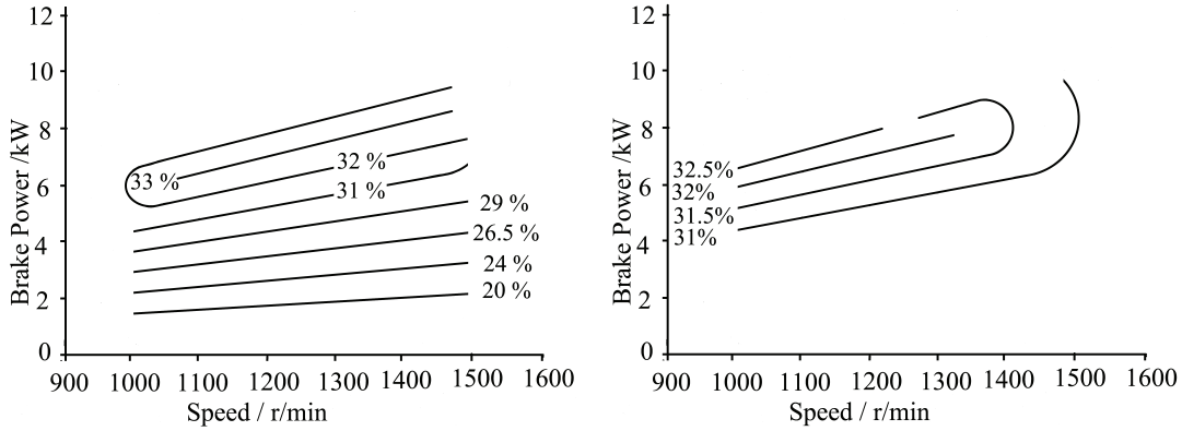
(a) Thermal Efficiency - Diesel
