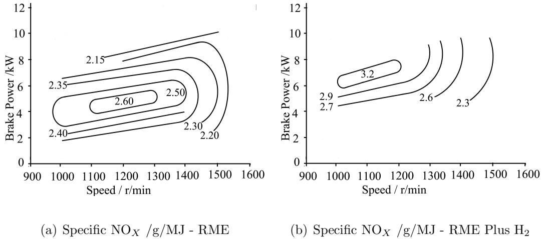
Figure 5.8. Experimentally obtained specific NO x emissions contours for RME baseline (a) and RME-H 2 dual fueling (b)
