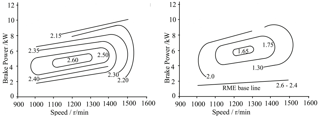
(a) Specific \text{NO}_x /g/MJ - RME
