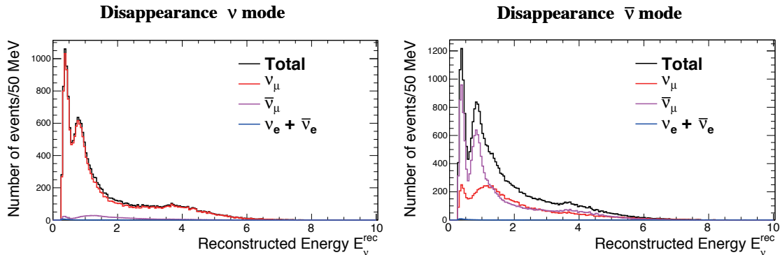
Fig. 12: Reconstructed neutrino energy distribution of the \nu_\mu candidate events.
