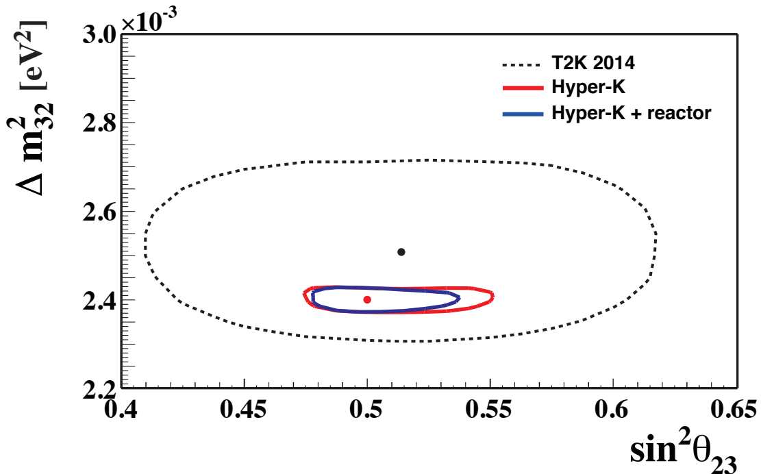
Fig. 23: The 90% CL allowed regions in the \sin^2 \theta_{23} - \Delta m_{32}^2 plane. The true values are \sin^2 \theta_{23} = 0.5 and \Delta m_{32}^2 = 2.4 \times 10^{-3} \text{ eV}^2 (red point). Effect of systematic uncertainties is included. The red (blue) line corresponds to the result with Hyper-K alone (with a reactor constraint on \sin^2 2\theta_{13} ). The dotted line is the 90% CL contour from T2K experiment [38] with the best fit values indicated by a black point.
