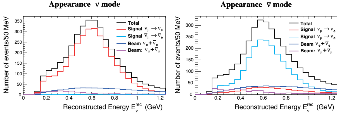
Fig. 11: Reconstructed neutrino energy distribution of the \nu_e candidate events. Normal mass hierarchy with \sin^2 2\theta_{13} = 0.1 and \delta_{CP} = 0 is assumed.
