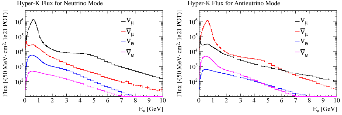
Fig. 8: The predicted Hyper-K neutrino fluxes from the J-PARC beam without oscillations. The neutrino enhanced beam is shown on the left and the antineutrino enhanced beam is shown on the right.
