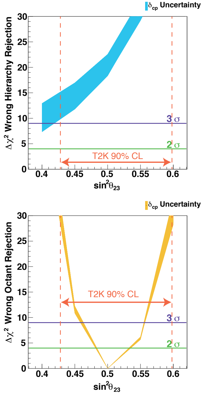
Fig. 25: Atmospheric neutrino sensitivities for a ten year exposure of Hyper-K assuming the mass hierarchy is normal. Top: the \Delta\chi^2 discrimination of the wrong hierarchy hypothesis as a function of the assumed true value of \sin^2\theta_{23} . Bottom: the discrimination between the wrong octant for each value of \sin^2\theta_{23} . The uncertainty from \delta_{CP} is represented by the thickness of the band. Vertical dashed lines indicate 90% confidence intervals of \sin^2\theta_{23} from the T2K measurement in 2014 [38].
