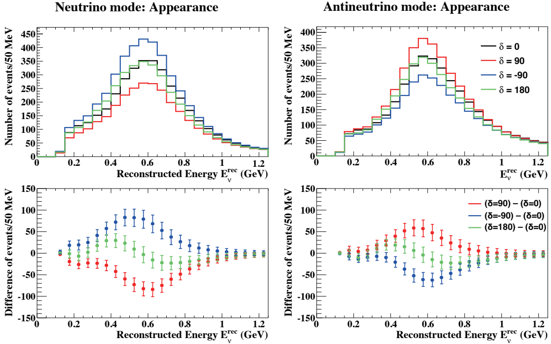
Fig. 13: Top: Reconstructed neutrino energy distribution for several values of \delta_{CP} . \sin^2 2\theta_{13} = 0.1 and normal hierarchy is assumed. Bottom: Difference of the reconstructed neutrino energy distribution from the case with \delta_{CP} = 0^\circ . The error bars represent the statistical uncertainties of each bin.
