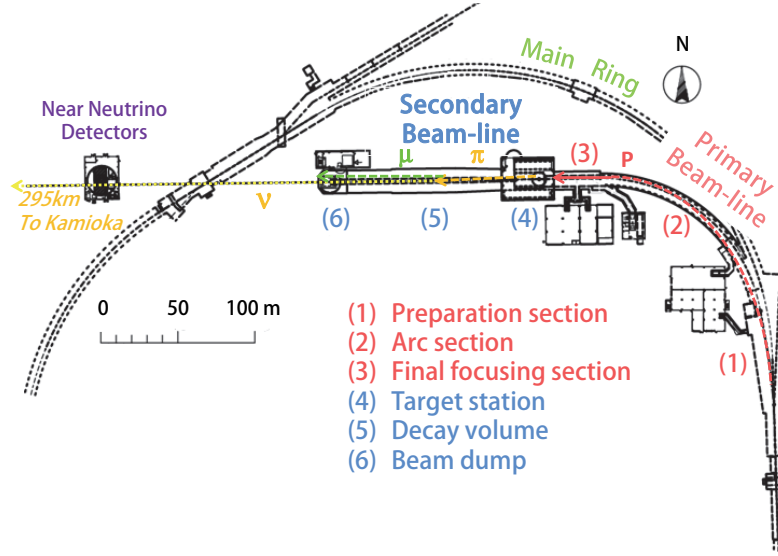
Fig. 2: The neutrino experimental facility (neutrino beamline) at J-PARC.
