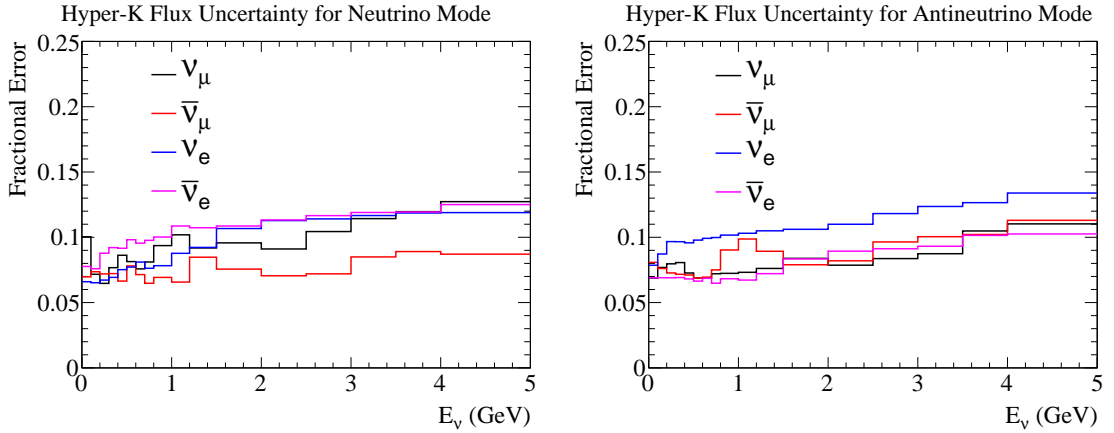
Fig. 9: The predicted uncertainty on the neutrino flux calculation assuming replica target hadron production data are available.
