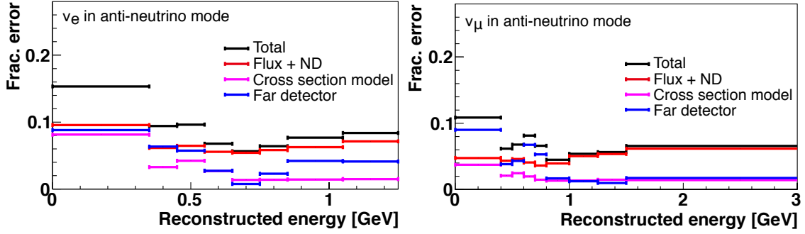
Fig. 16: Fractional error size for the appearance (left) and the disappearance (right) samples in the anti-neutrino mode. Black: total uncertainty, red: the flux and cross-section constrained by the near detector, magenta: the near detector non-constrained cross section, blue: the far detector error.
