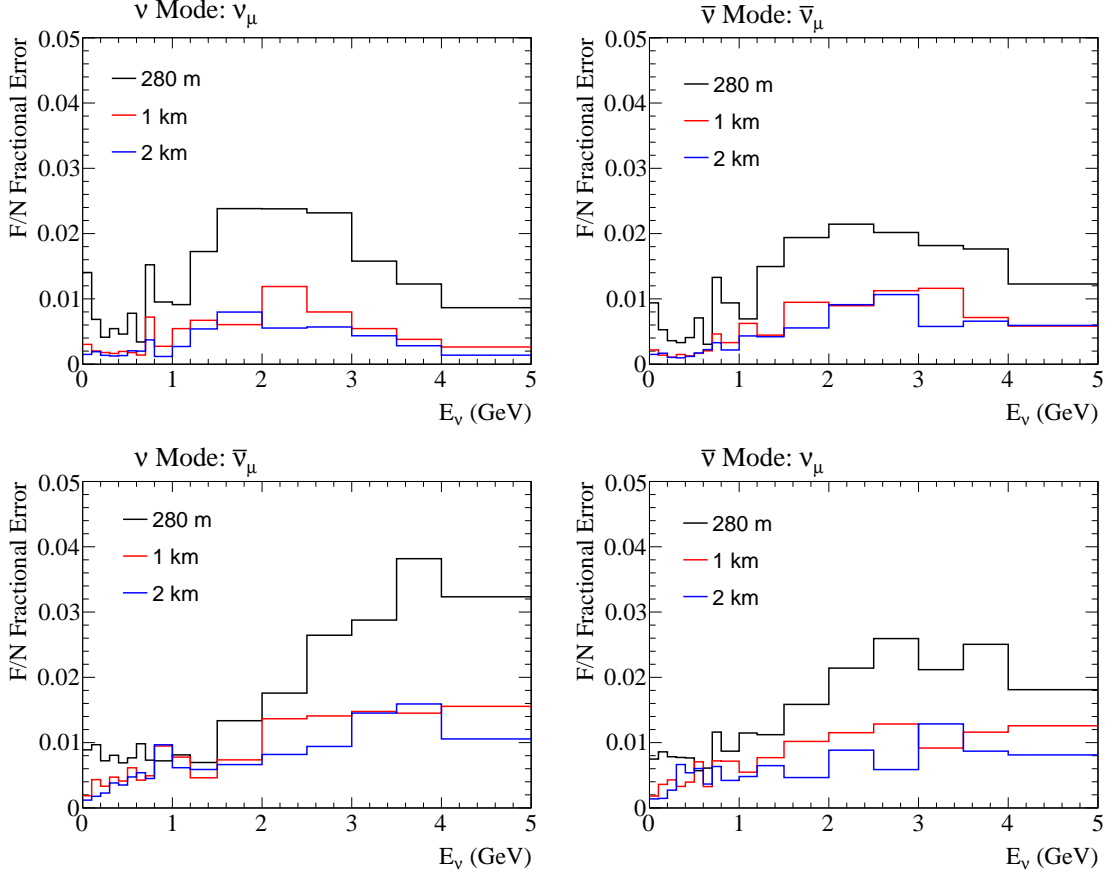
Fig. 10: The uncertainty on the far-to-near flux ratio for near detectors at 280 m, 1 km and 2 km. Left: neutrino enhanced beam. Right: antineutrino enhanced beam. Top: the focused component of the beam. Bottom: the defocused component of the beam.
