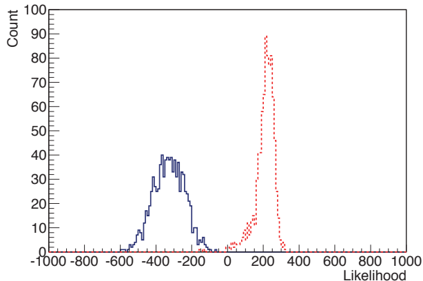
Fig. 5: PID likelihood functions for electron (blue solid histogram) and \mu (red dashed histogram) with 500 \text{ MeV}/c momentum. A negative (positive) value indicates electron-like ( \mu -like) particle.
