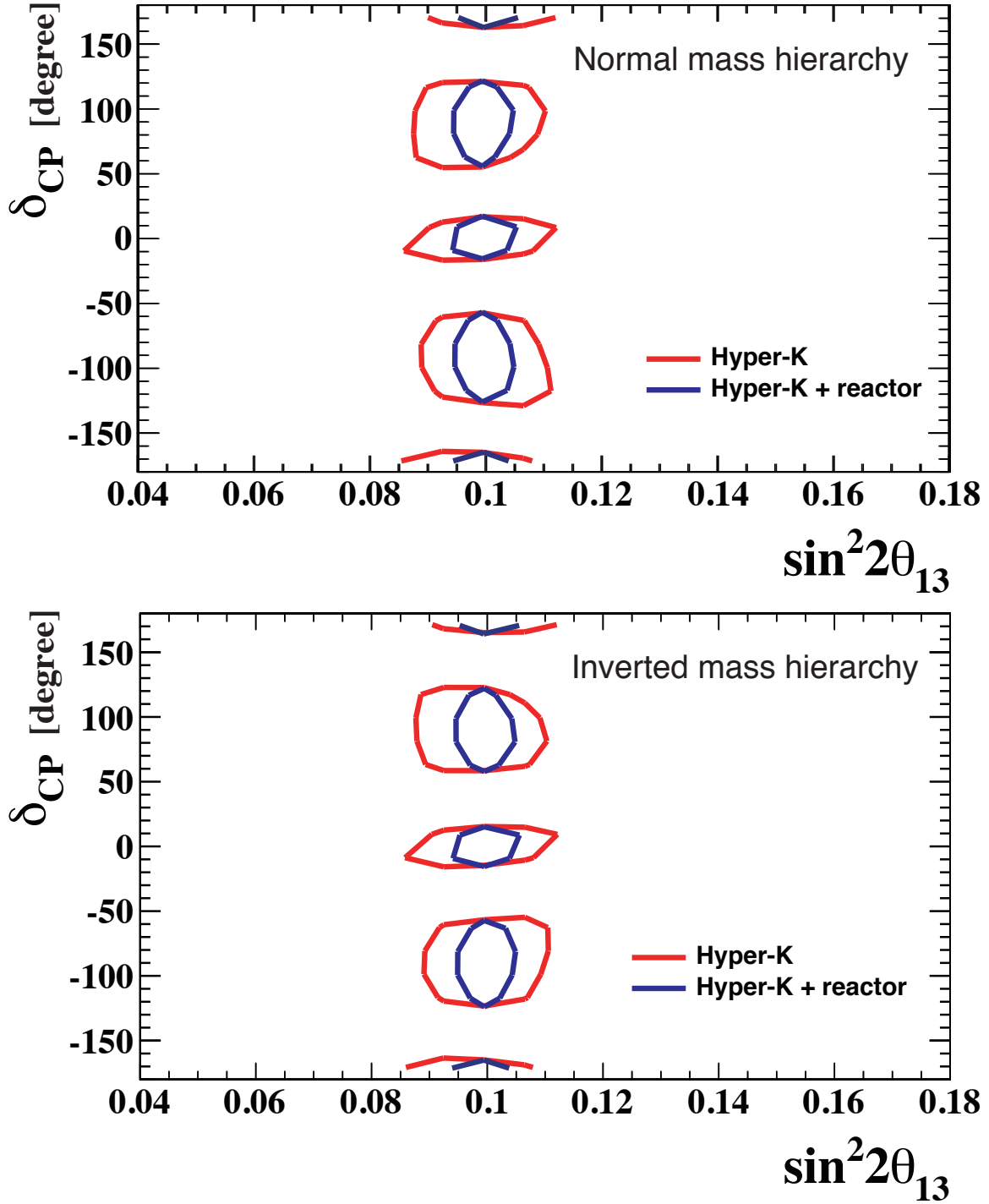
Fig. 18: The 90% CL allowed regions in the \sin^2 2\theta_{13} - \delta_{CP} plane. The results for the true values of \delta_{CP} = (-90^\circ, 0, 90^\circ, 180^\circ) are overlaid. Top: normal hierarchy case. Bottom: inverted hierarchy case. Red (blue) lines show the result with Hyper-K only (with \sin^2 2\theta_{13} constraint from reactor experiments).
