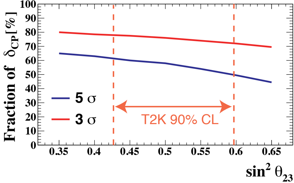
Fig. 22: Fraction of \delta_{CP} for which \sin \delta_{CP} = 0 can be excluded with more than 3\sigma (red) and 5\sigma (blue) significance as a function of the true value of \sin^2 \theta_{23} , for the normal hierarchy case. Vertical dashed lines indicate 90% confidence intervals of \sin^2 \theta_{23} from the T2K measurement in 2014 [38].
