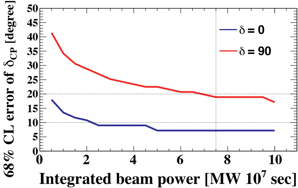
Fig. 21: Expected 68% CL uncertainty of \delta_{CP} as a function of integrated beam power.
