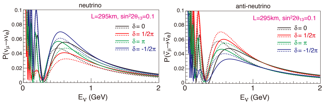
Fig. 6: Oscillation probabilities as a function of the neutrino energy for \nu_\mu \rightarrow \nu_e (left) and \bar{\nu}_\mu \rightarrow \bar{\nu}_e (right) transitions with L=295 \text{ km} and \sin^2 2\theta_{13} = 0.1 . Black, red, green, and blue lines correspond to \delta_{CP} = 0, \frac{1}{2}\pi, \pi, and -\frac{1}{2}\pi , respectively. Solid (dashed) line represents the case for a normal (inverted) mass hierarchy.
