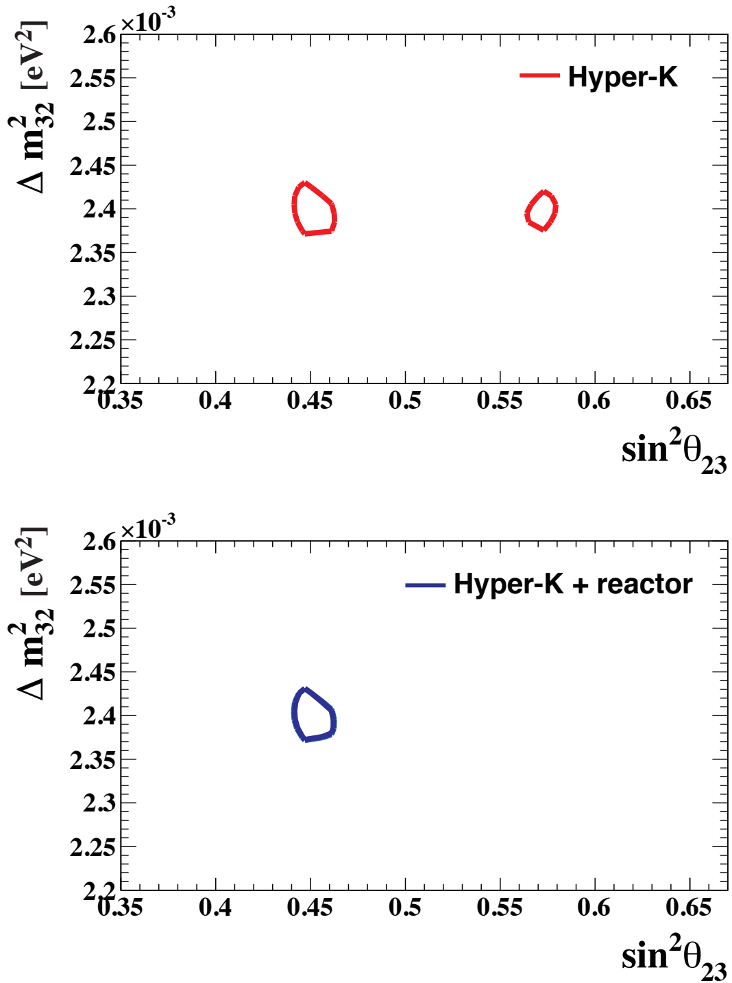
Fig. 24: 90% CL allowed regions in the \sin^2 \theta_{23} - \Delta m_{32}^2 plane. The true values are \sin^2 \theta_{23} = 0.45 and \Delta m_{32}^2 = 2.4 \times 10^{-3} eV 2 . Effect of systematic uncertainties is included. Top: Hyper-K only. Bottom: With a reactor constraint.
