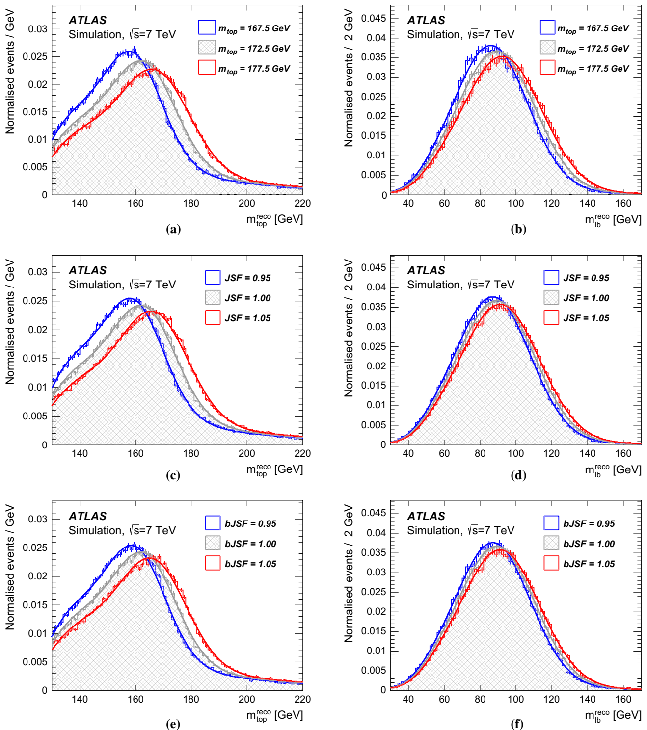
Fig. 2 Distributions of m_{\text{top}}^{\text{reco}} in the t\bar{t} \rightarrow \text{lepton}+\text{jets} channel (left) and m_{\text{lb}}^{\text{reco}} in the t\bar{t} \rightarrow \text{dilepton} channel (right) and their template parameterisations for the signal, composed of simulated t\bar{t} and single top quark production events. The expected sensitivities of m_{\text{top}}^{\text{reco}} and m_{\text{lb}}^{\text{reco}} are shown for events with at least two (or exactly two) b -tagged jets. Figures a and b report the distributions for different values of the input
