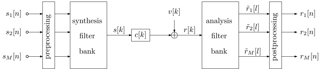
FIGURE 1. Block diagram of a general FBMC system.
