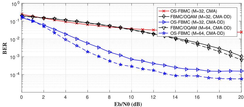
FIGURE 2. BER performances comparison of FBMC/OQAM to OS-FBMC
