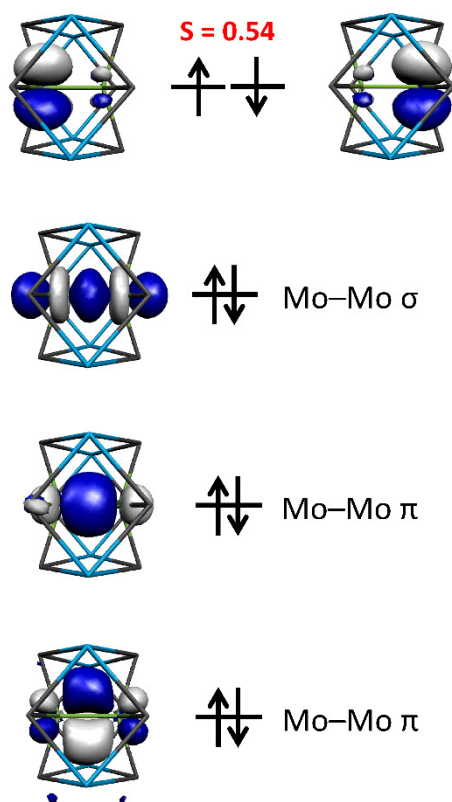
Figure 3. Qualitative MO scheme depicting the ordering of the frontier Mo d orbitals for 5 showing three Mo–Mo bonds and one pair of corresponding MOs that constitute the BS(1,1) S = 0 solution. The S-value indicates the calculated overlap between
