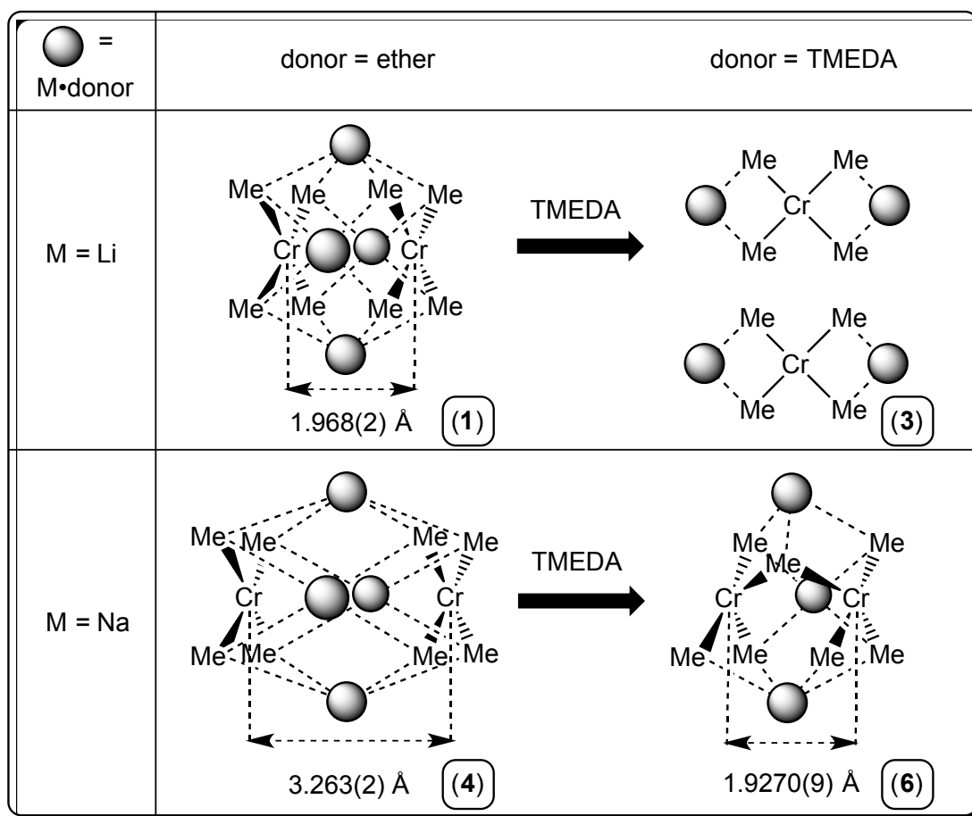
Scheme 2. Highlighting the reactivity contrast of the lithium and sodium octamethylchromate complexes towards the diamine TMEDA.
