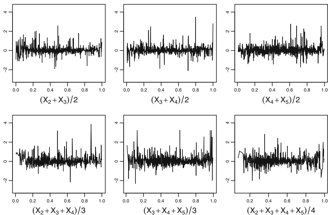
Fig. 10 Evolving paths of the difference between the true log-likelihood and the estimated log-likelihood (trees T_3 , T_4 and T_5 )
