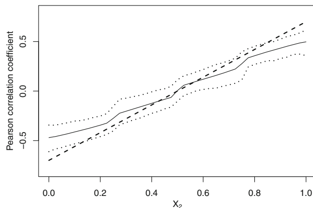
Fig. 9 The true and estimated correlation coefficients, varying with the value of the conditioning variable X_2 . The true correlation coefficient is shown as a dashed curve , the average of the estimates taken over 100 Monte Carlo samples is displayed by the solid curve and the 90% Monte Carlo confidence intervals are given by dotted curves
