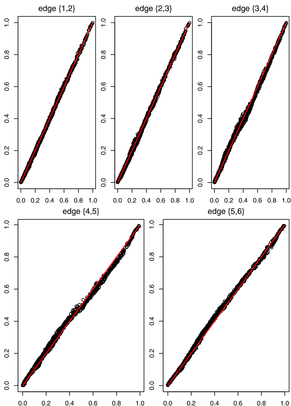
Fig. 11 Q–Q plots for the five copulas in tree T_1 . The x -axis represents the quantiles of the simulated data calculated using \hat{H}_0(u, w) , and the y -axis represents the quantiles of the simulated data calculated using \hat{H}_1(u, w)
