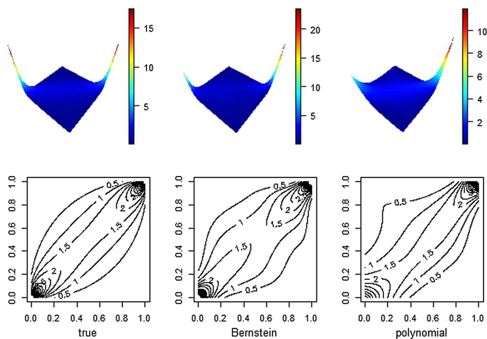
Fig. 5 Surface plots and contour plots of the true bivariate t -copula with \rho = 0.7 (left), of the minimally informative copula having five Bernstein basis functions (middle), and of the minimally informative copula having five polynomial basis functions (right)
