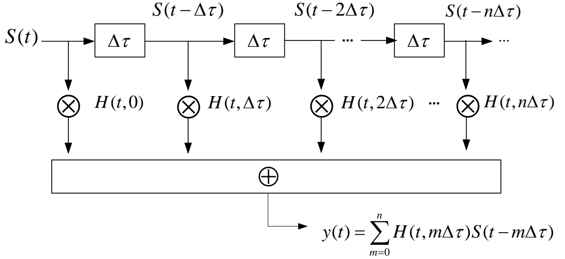
FIGURE 4.6: The tap-delay line based channel simulator.
