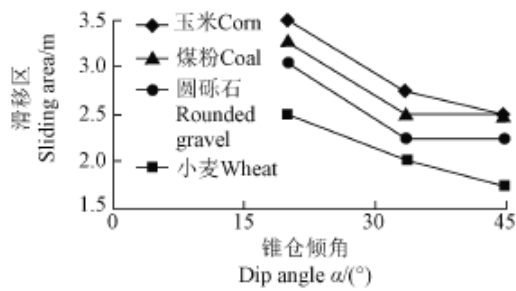
图4 玉米、煤粉、圆砾石和小麦滑移区随锥仓倾角变化图 Fig.4 Sliding area change tendency with dip angle
