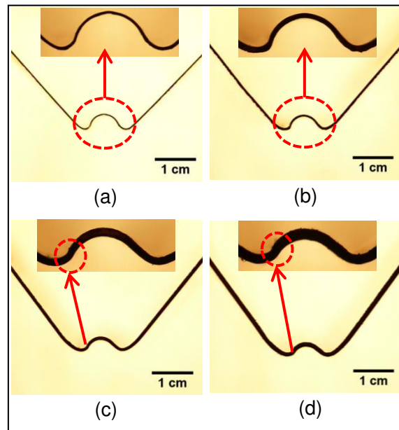
Figure 9. W-shaped micro-bent parts annealed under 650^{\circ}\text{C} with three-hour holding time: (a) t = 25\ \mu\text{m} , bending angle = 84.253^{\circ} , (b) t = 50\ \mu\text{m} , bending angle = 80.343^{\circ} , (c) t = 75\ \mu\text{m} , bending angle = 75.339^{\circ} , and (d) t = 100\ \mu\text{m} , bending angle = 75.056^{\circ} .
