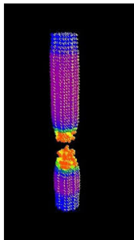
Fig. 4. A meshless discretization for a peridynamic model of a cylindrical bar under tension loading [18]
