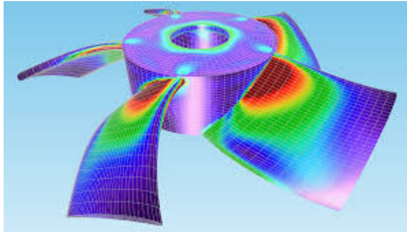
Fig. 2. Finite element analysis of a cooling fan (Comsol) [1]
