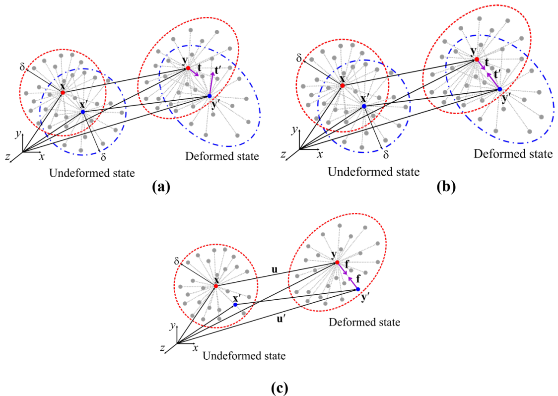
Fig. 3. Various peridynamic formulations; (a) non-ordinary state based peridynamics, b) ordinary state based peridynamics and (c) bond based peridynamics [5]
