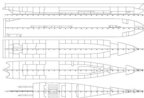
Figure 4: General Arrangement
