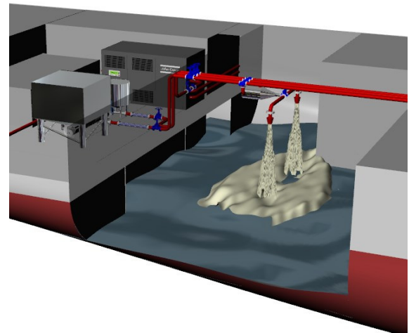
Figure 1 - System Representation
