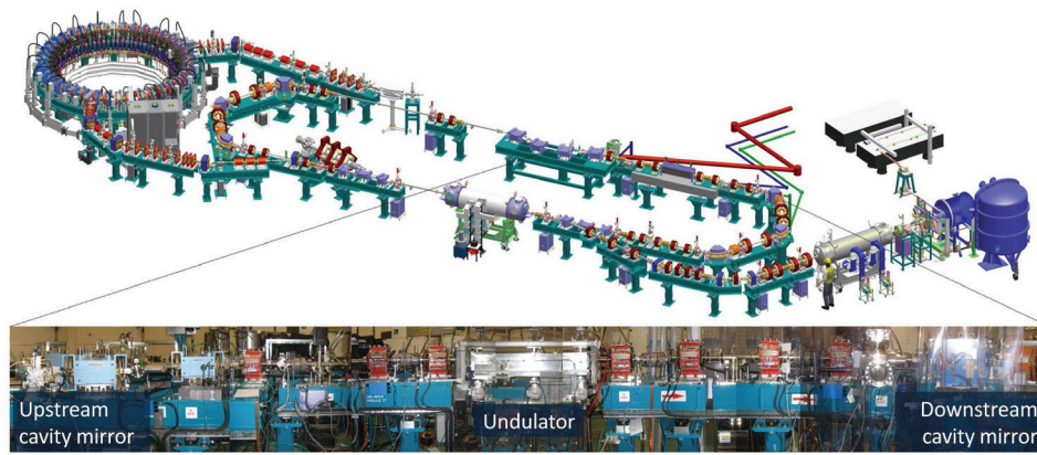
Figure 1: Layout of the ALICE facility and FEL line.
