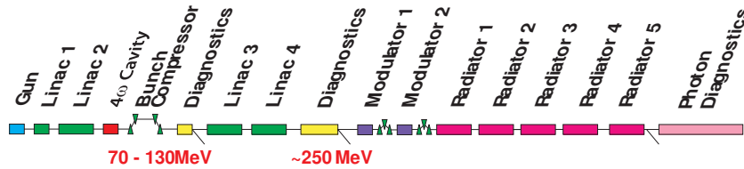
Figure 3: CLARA Schematic layout.
