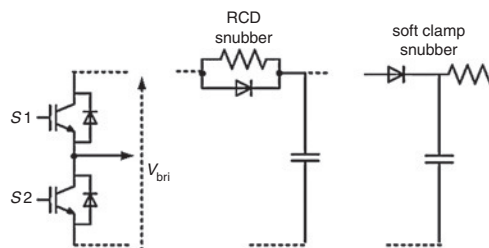
Fig. 3 Conventional snubber networks [5]
