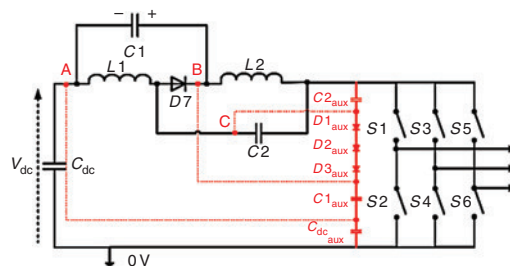
Fig. 4 Quasi-Z-source inverter with proposed snubber
