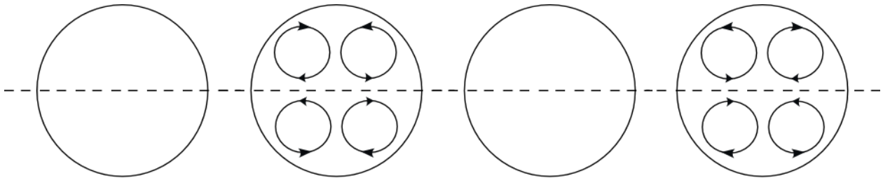
Figure 15: Snapshots of velocity field in the cross section z=0 at two instants during the period \tau of oscillation (case C): a) t=t_0 , b) t=t_0+\tau/2 ( \tau=2\pi/\omega ).
