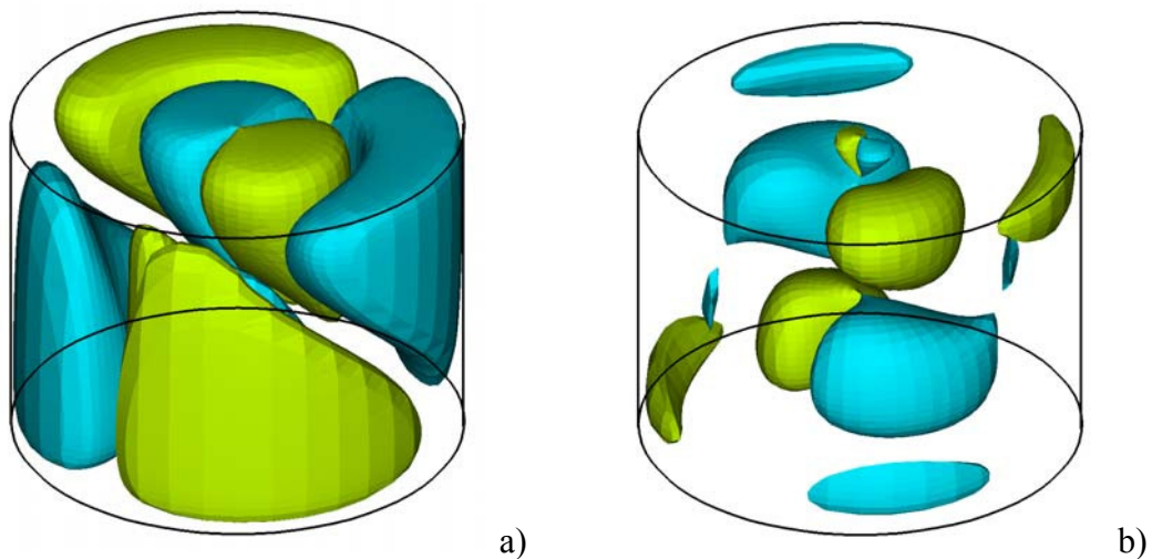
Figure 17: Snapshots of 3D isosurfaces of azimuthal velocity component w ( w = \pm 1 ) for the same conditions considered in Figure 12: a) t=t_0 , b) t=t_0+\tau/4 .
