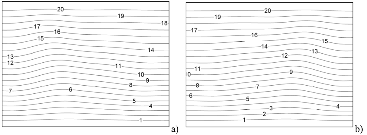
Figure 5: Snapshots of temperature distribution in the meridional plane xz ( \varphi=0 ) at two instants during the period \tau of oscillation (case A, contour legend: level 1 \rightarrow T=-0.45 , level 20 \rightarrow T=0.45 , \Delta_{\text{level}} \rightarrow 0.05 ): a) t=t_0 , b) t=t_0+\tau/2 ( \tau=2\pi/\omega ).
