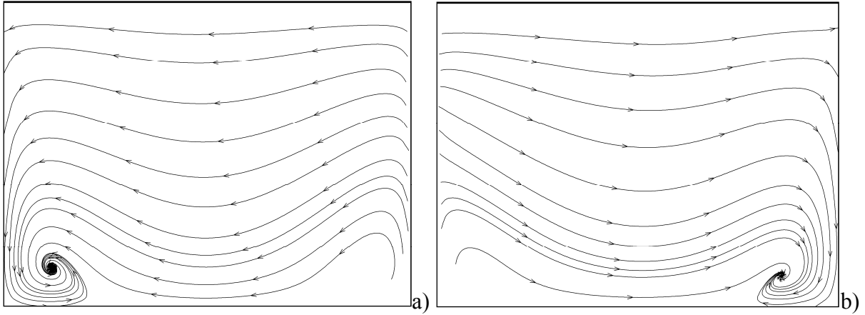
Figure 9: Snapshots of velocity field in the meridional plane xz ( \varphi=0 ) at two instants during the period \tau of oscillation (case A): a) t=t_0 , b) t=t_0+\tau/2 ( \tau=2\pi/\omega ).
