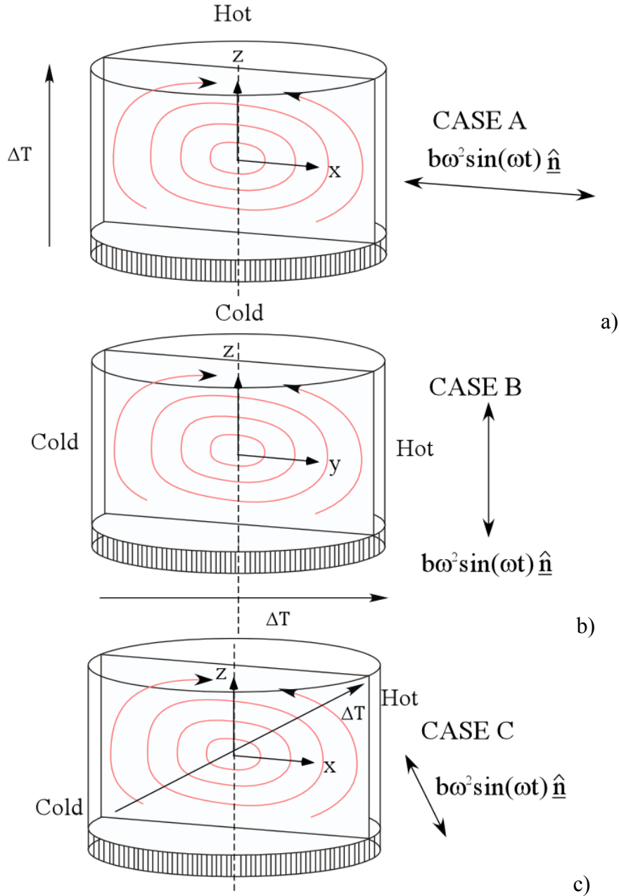
Figure 1: Sketch of configuration under investigation: a) Cylinder with differentially heated ends and adiabatic sidewall subjected to vibrations perpendicular to its axis, b) Cylinder with insulated ends and nonisothermal sidewall (temperature varying as a sinusoidal function of the azimuthal angle) subjected to vibrations parallel to its axis, c) Cylinder with temperature varying on the boundary along both the axial and the azimuthal direction and vibrations perpendicular to the imposed temperature gradient.
