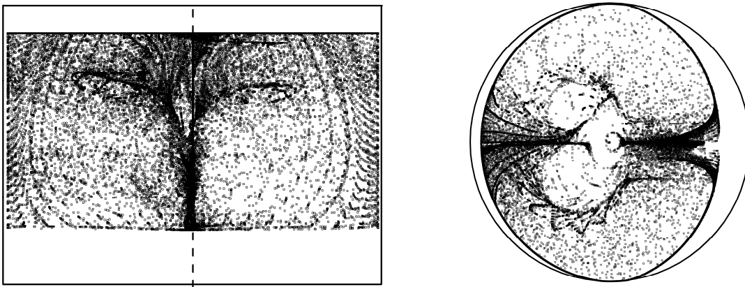
Figure 18: Snapshot of particle aggregates (lateral and top views, case C).
