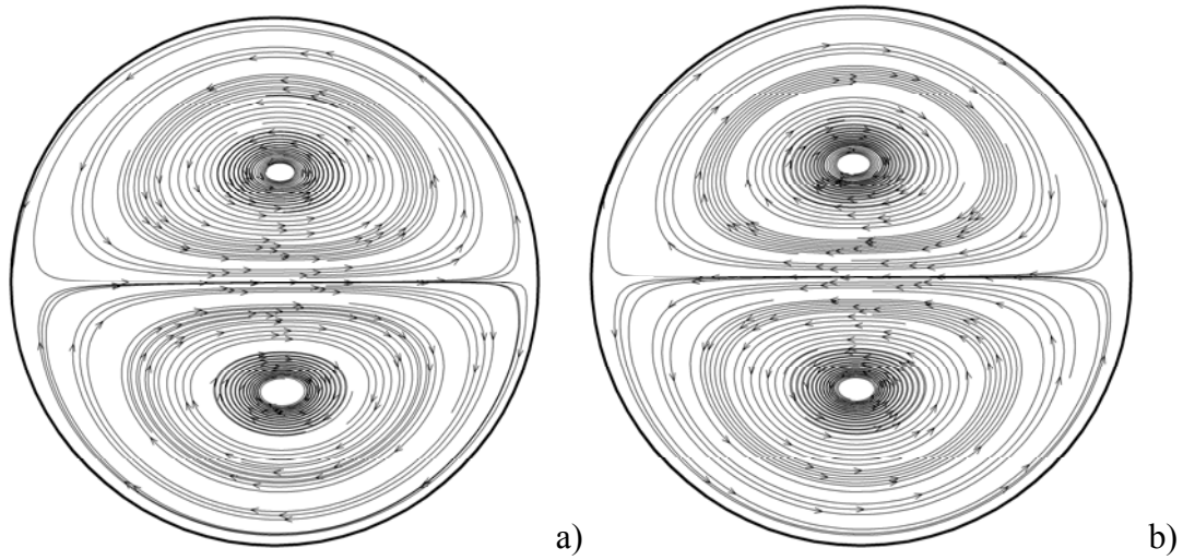
Figure 6: Snapshots of velocity field in the cross section z=0 at two instants during the period \tau of oscillation (case A): a) t=t_0 , b) t=t_0+\tau/2 ( \tau=2\pi/\omega ).
