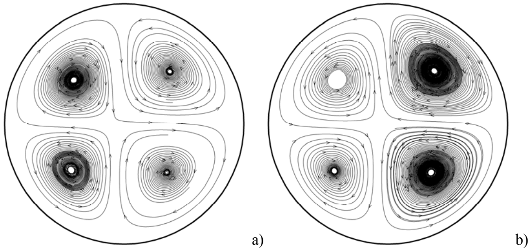
Figure 15: Snapshots of velocity field in the cross section z=0 at two instants during the period \tau of oscillation (case C): a) t=t_0 , b) t=t_0+\tau/2 ( \tau=2\pi/\omega ).
