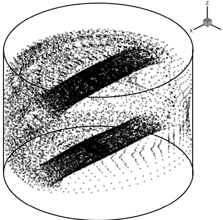
Figure 12: 3D snapshots of particle aggregates (case B, t=5.6 \times 10^{-1} ).
