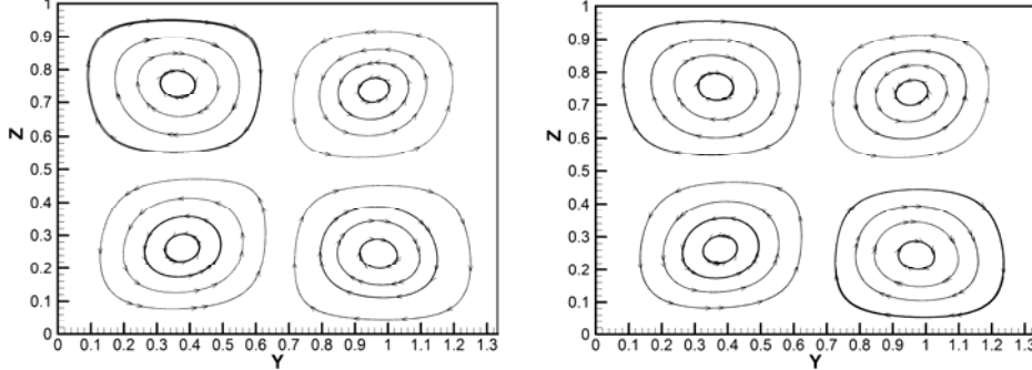
Figure 4: Classical "quadrupolar" flow field in the yz plane obtained by a) time-averaging of the oscillatory solution, b) integration of the Gershuni's equations (cylinder with insulated ends and nonisothermal sidewall with temperature varying as a sinusoidal function of the azimuthal angle, vibrations along the z axis, Pr=8 , A=0.75 , \omega=1 \times 10^3 , Ra_\omega=1.58 \times 10^4 ).
