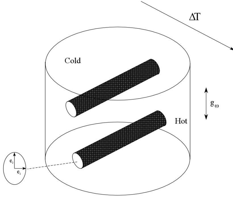
Figure 3: Sketch of cylindrical enclosure, related thermal boundary conditions, imposed vibrations and emerging particulate aggregates.
