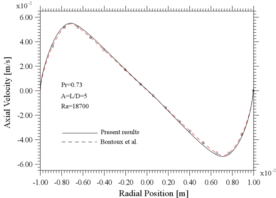
Figure 2: Comparison with the results reported by Bontoux et al. [16]: differentially heated horizontal cylinder with L = 10^{-1} m, A=5 , Pr=0.73 , Ra=1.87 \times 10^4 ( N_z \times N_r \times N_\phi mesh 65 \times 16 \times 32 ).
