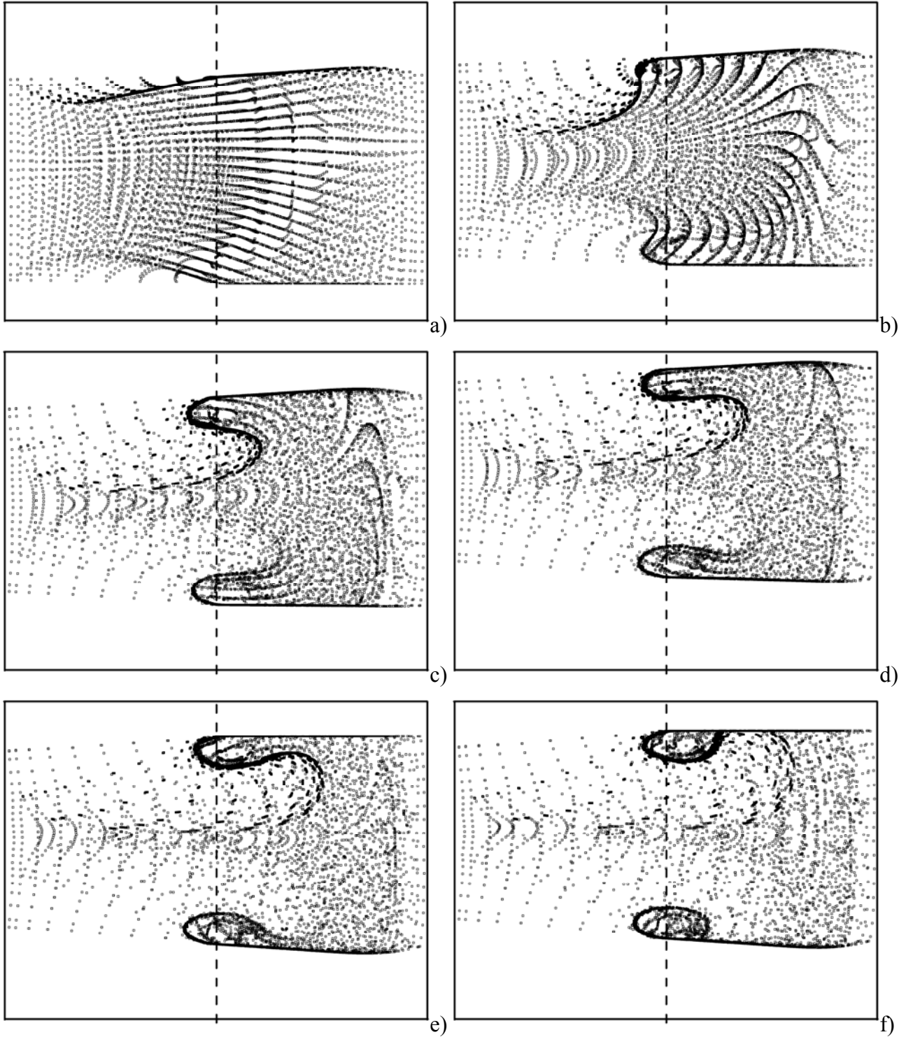
Figure 13: Lateral view (from the x axis perspective) of particle aggregates as a function of time (case B): a) t=2.7 \times 10^{-2} , b) t=9.5 \times 10^{-2} , c) t=1.6 \times 10^{-1} , d) t=1.9 \times 10^{-1} , e) t=2.24 \times 10^{-1} , f) t=2.56 \times 10^{-1} .
