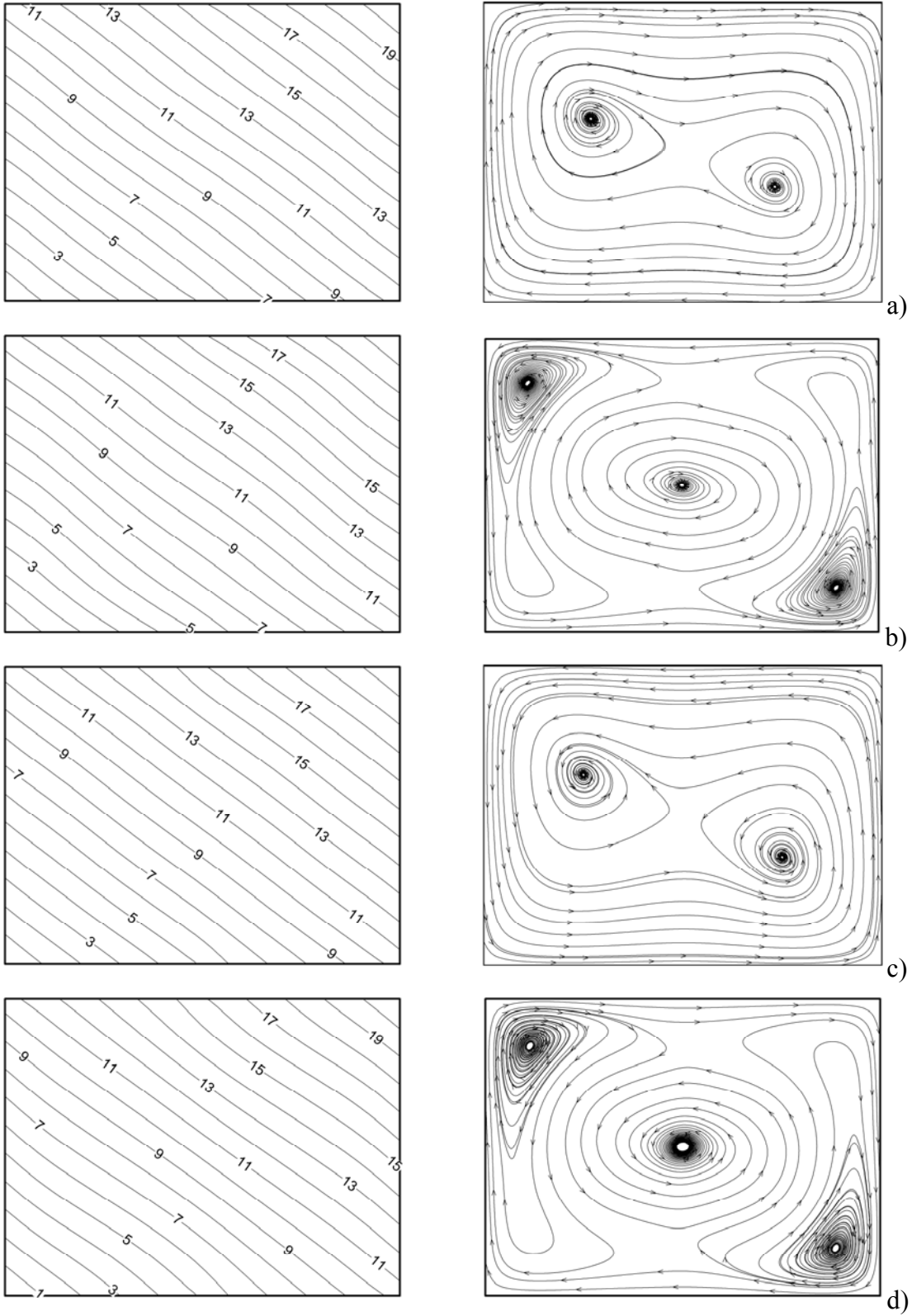
Figure 14: Snapshots of temperature distribution (left) and velocity field (right) in the meridional plane xz ( \varphi=0 ) at four instants evenly space in time during the period \tau of oscillation (case C, contour legend: level 1 \rightarrow T=-0.45 , level 20 \rightarrow T=0.45 , \Delta_{\text{level}} \rightarrow 0.05 ): a) t = t_0 , b) t = t_0 + \tau/4 , c) t = t_0 + \tau/2 , d) t = t_0 + 3\tau/4 ( \tau = 2\pi/\omega ).
