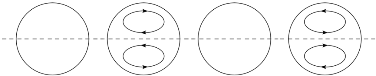
Figure 7: Sequence (sketch) showing the evolution of vibrations-induced convective cells in the generic cross section z=\text{const} during one period of oscillation (case A).
