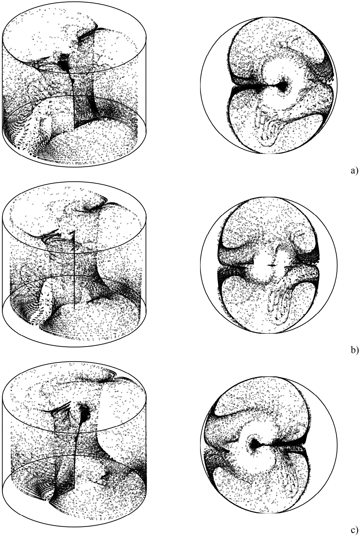
Figure 10: 3D snapshots of particle aggregates (case A): a) t=t_0 , b) t=t_0+\tau/4 , c) t=t_0+\tau/2 ( t_0=1.4 \times 10^{-1} , \tau=2\pi/\omega ).
