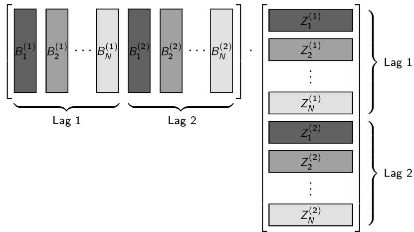
Figure 4. Sub-block partitions.
