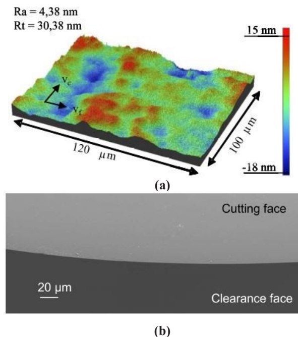
Figure 1. Ultrasonic-assisted diamond machining on hardened steel: (a) Machined surface topography; (b) SEM image of the monocrystalline diamond tool after machining [4]
