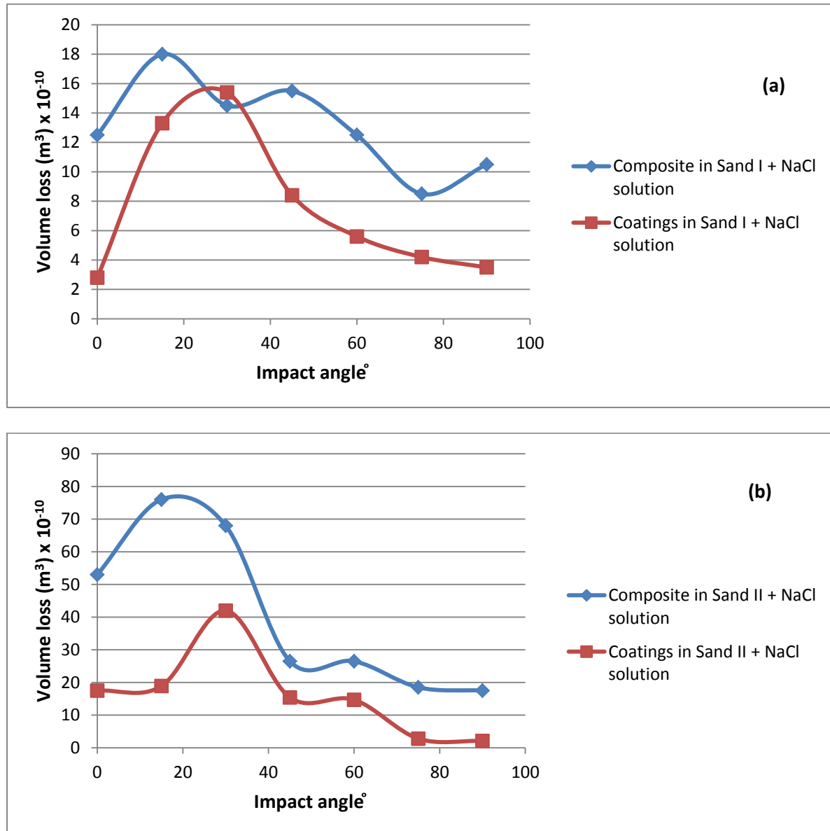
Fig. 7 – Volume loss comparison of composite and coatings specimens as a function of impact angle in NaCl solution (a) in Sand I + NaCl solution slurry (b) in Sand II + NaCl solution slurry.
