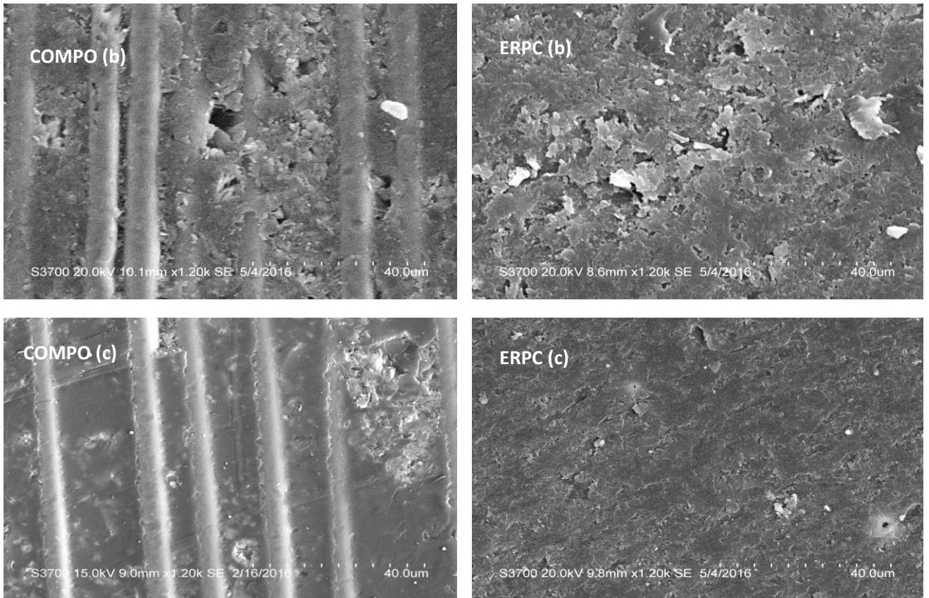
Fig. 8 – SEM micrographs of the exposed surfaces of composite and composite base polymeric coatings in NaCl solution + Sand I, (a) at impact angle 15°, (b) at impact angle 30°, and (c) at impact angle 60°.
