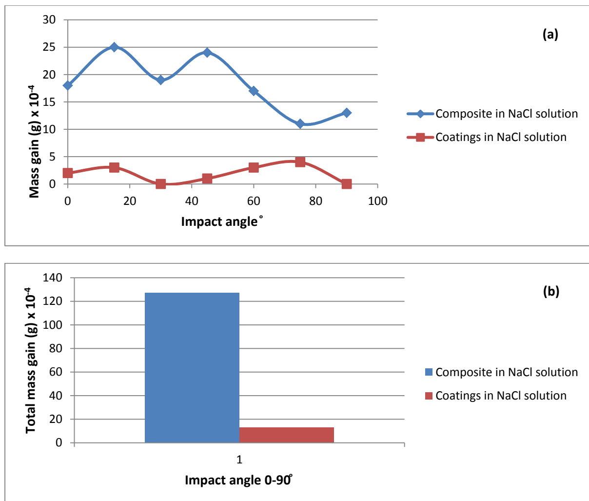
Figure 3– Mass gain of composite and coatings specimens as a function of impact angle in NaCl solution (a) at various impact angles (b) total mass gain in NaCl solution.
