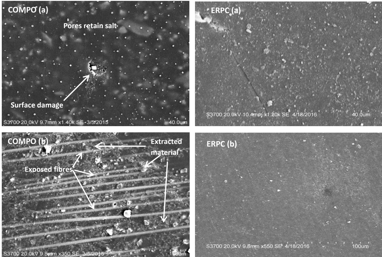
Fig. 6 – Exposed surfaces after a test in NaCl solution at 60° angle of attack, composite: COMPO (a) site 1, COMPO (b) site 2; coatings: ERPC (a) site 1 and ERPC (b) site 2.
