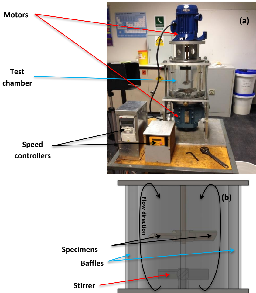
Figure 2 – (a) Slurry pot testing rig and (b) Test chamber
