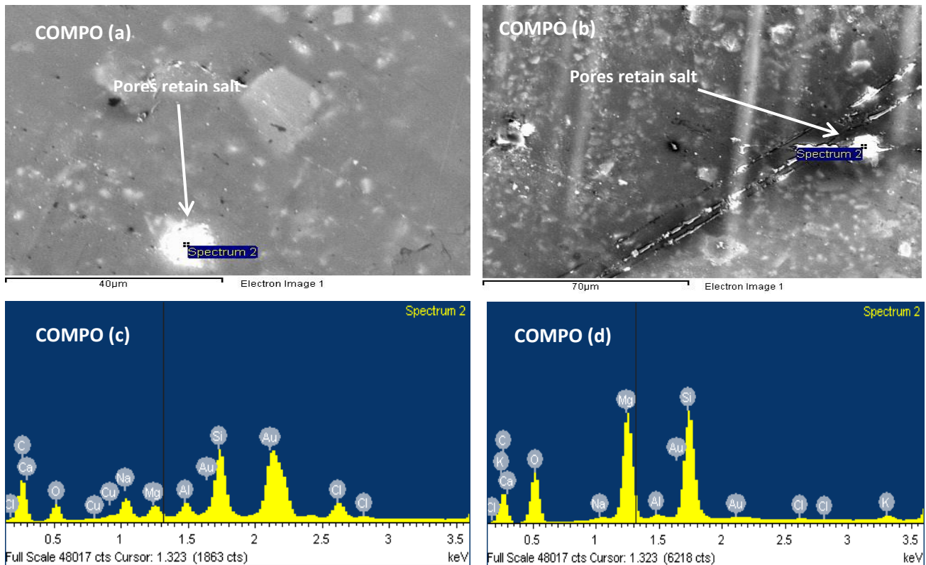
Fig. 4 – Composite exposed surface SEM and EDX after a test in NaCl solution at 60° angle of attack (a) site 1, (b) site 2, (c) EDX analysis of (a), and (d) EDX analysis of (b).
