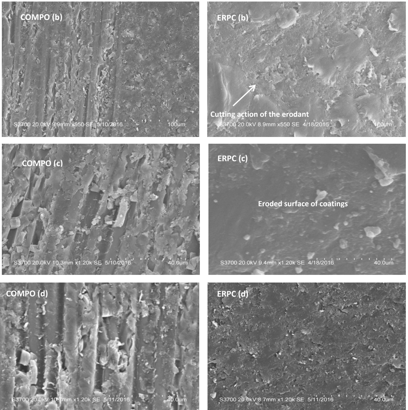
Fig. 9 – SEM micrographs of the exposed surfaces of composite and composite base polymeric coatings in NaCl solution + Sand II, (a) at impact angle 15^\circ , (b) at impact angle 30^\circ , (c) at impact angle 60^\circ , and (d) at impact angle 75^\circ .
