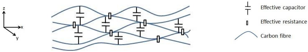
Figure 2: Simplified 2-dimensional diagram of the x (along fibre) and z (transverse) electrical model of a section of unidirectional CFRP.
