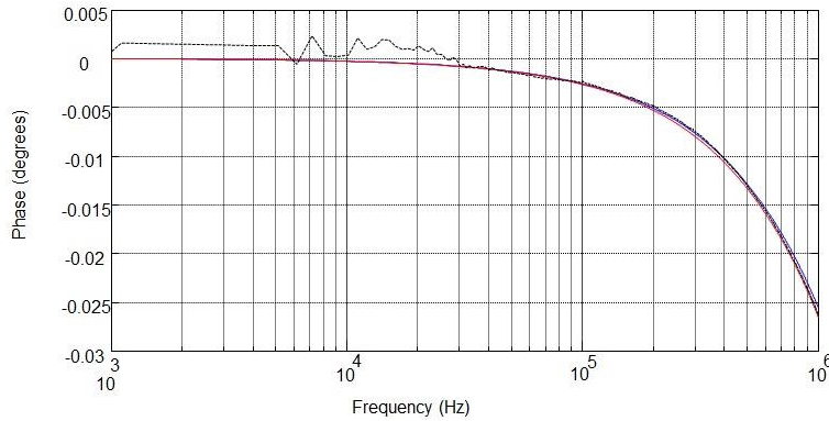
Figure 6: Comparison of theoretical and experimental measured frequency response of the impedance in the z-direction.
