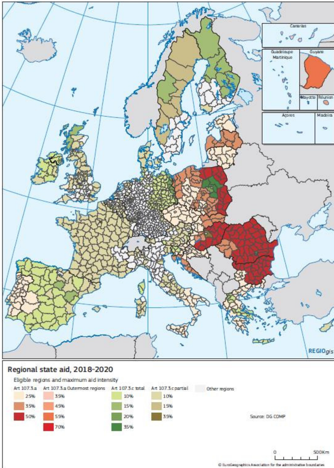
Figure 21: Regional aid ceilings 2018-20
