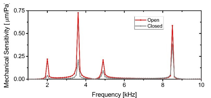
Fig. 4: Simulated mechanical frequency response at normal incidence for closed and open backside holder.
