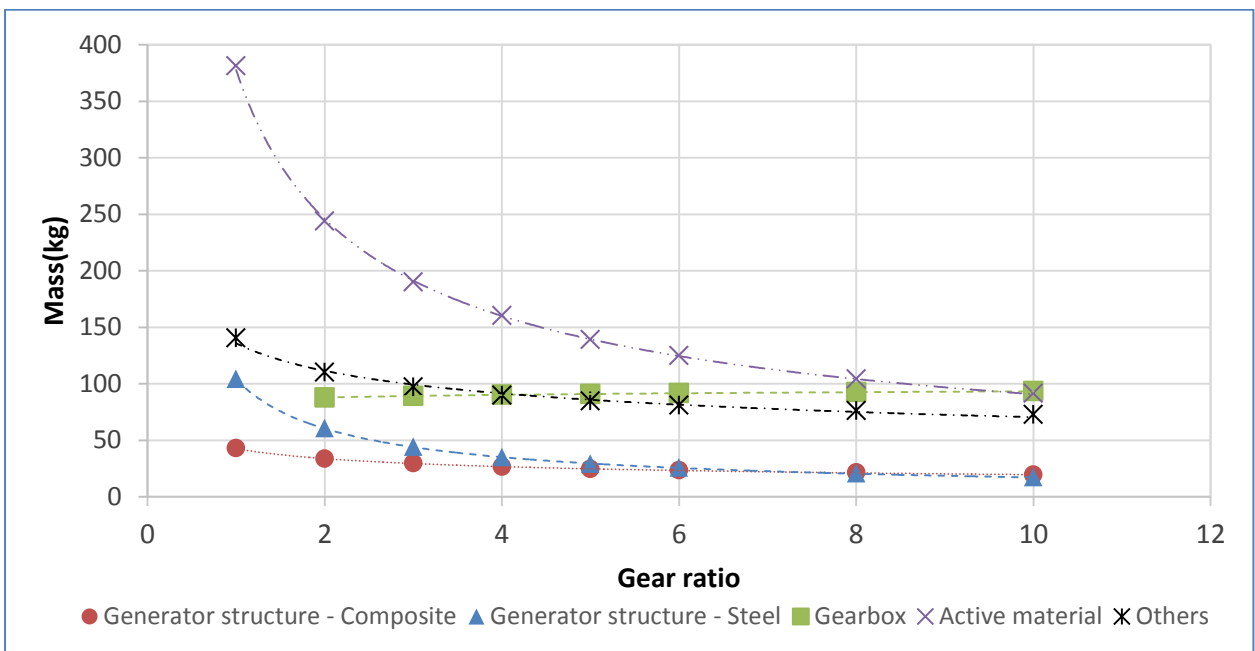
Figure 9: Breakdown of mass for the generator models
