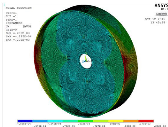
Figure 6: Rotor composite structure highlighting deformation in radial direction
