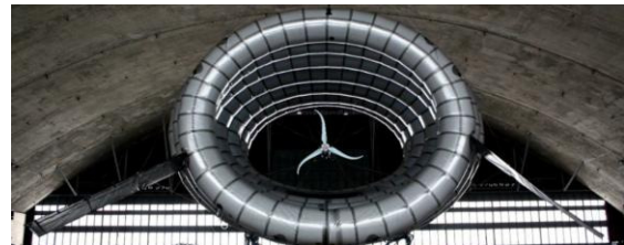
Figure 1: Buoyant airborne wind turbine (BAT) [1]
