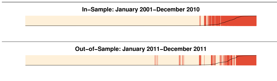
FIGURE 1. Separation plots for CRISP Model Prediction of UCDP Data
