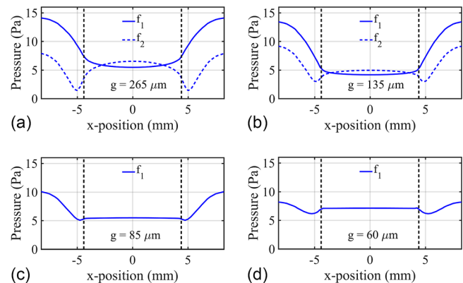
FIG. 4. Predicted pressure amplitudes evaluated along the intersection of the xy - and xz - planes as shown in the inset in Fig. 3, for (a) g = 265 \mu\text{m} , (b) g = 135 \mu\text{m} , (c) g = 85 \mu\text{m} , and (d) g = 60 \mu\text{m} . Pressure amplitudes for frequency of the lowest ( f_1 ) and highest ( f_2 ) order resonances, respectively, in (a) and (b) and the frequency of the single resonance supported by the structure in (c) and (d). (Black dashed lines indicate the position of the edge of the pipe.)
