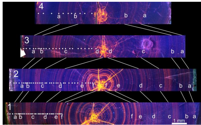
Figure 1: Cathodoluminescence pattern for sections through the rostrum adjacent to geochemical transects one to four. Letters “a” to “f” correlated between the profiles with white lines as well as white dots indicate arbitrarily chosen marker bands for illustration of differences in precipitation rate (see also Fig. 2). Note the increasing distance of marker bands from profile one to four.
