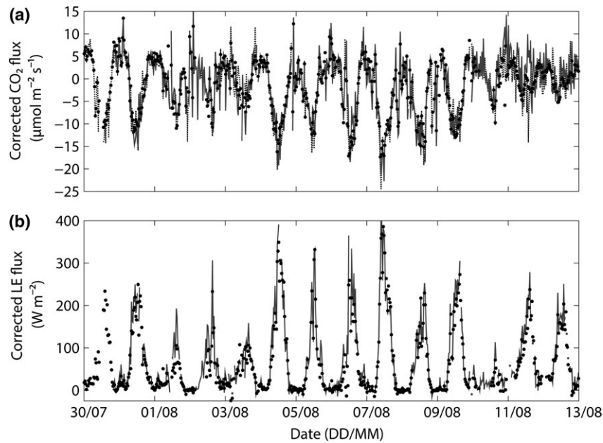
Fig. 6 A 2-week selection of half-hourly corrected CO 2 and LE fluxes. The LI-7500 is shown as dots, the GMP343 #1 is shown with a dashed line and GMP343 #2/HH-4000 is shown with solid grey line.
