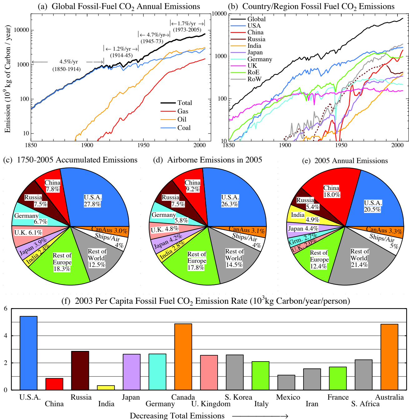
Figure 9. Fossil fuel annual emissions in terms of (a) fuel type, and (b) source country or region. (c) is accumulated 1750-2005 emissions by source region, (d) is the contribution to anthropogenic CO 2 remaining in the air in 2005 based on an analytic fit to the Bern carbon cycle model, (e) is 2005 emissions, and (f) is per capita emissions of the 15 largest sources in 2003. Data sources: Carbon Dioxide Information Analysis Center, Oak Ridge National Laboratory for 1751-2003 and British Petroleum [2006] for 2004-2005. Data for Russia are 60% of USSR for 1850-1991 and Russian Federation thereafter.
