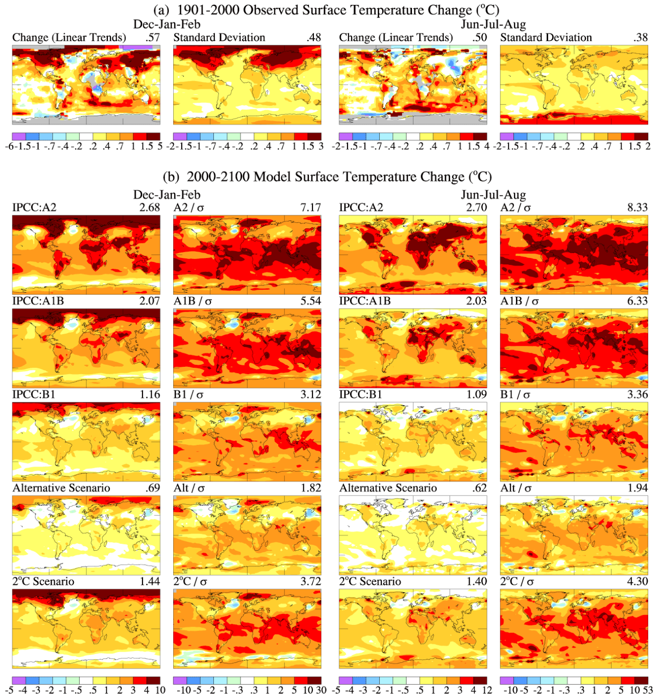
Figure 4. (a) Observed seasonal (DJF and JJA) surface temperature change in the past century based on local linear trends and the standard deviation about the local 100-year mean temperature, (b) simulated 21 st century seasonal temperature change for five GHG scenarios and the ratio of the simulated change to the observed 20 th century standard deviation.
