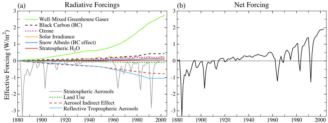
Figure 1. Effective global climate forcings ( F_e ) employed in our global climate simulations, relative to their values in 1880. Use of F_e avoids exaggerating the importance of BC and O_3 forcings.
