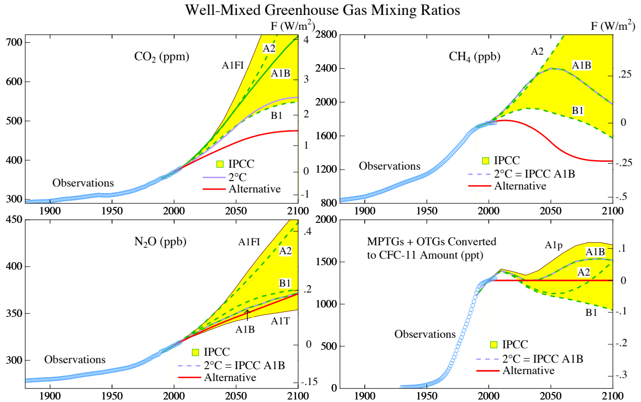
Figure 2. Observed greenhouse gas amounts as tabulated by Hansen and Sato [2004] and scenarios for the 21st century. Colored area delineates extreme IPCC [2001] scenarios. Alternative and 2°C scenarios are from Table 2 of Hansen and Sato [2004]. MPTGs and OTGs are Montreal Protocol trace gases and other trace gases [ Hansen and Sato , 2004]. Forcings on right hand scales are adjusted forcings, F_a , relative to values in 2000.
