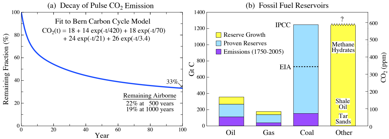
Figure 10. (a) Decay of a small pulse of \text{CO}_2 added to today's atmosphere, based on analytic approximation to the Bern carbon cycle model [Joos et al. , 1996; Shine et al. , 2005], (b) fossil fuel emissions to date based on sources in Figure 9, and proven reserves and estimated economically recoverable reserve growth based on EIA [2005] and, in the case of coal, IPCC [2001].
