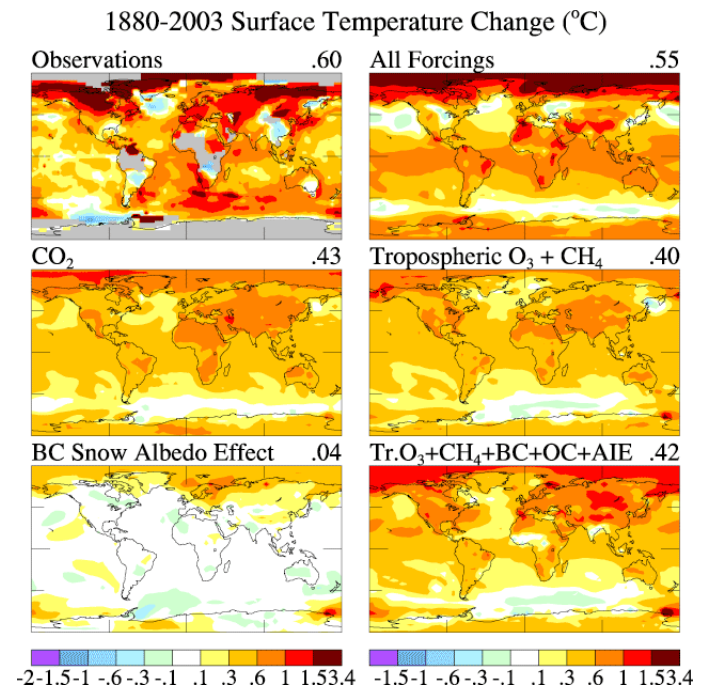
Figure 5. Surface temperature change based on local linear trends for observations and for simulations that employ different combinations of transient 1880-2003 forcings. CH 4 forcing includes its indirect effect on stratospheric H 2 O. Snow albedo effect has 1880-2003 Fa ~ 0.05 W/m 2 . Results in lower right include direct effects of black carbon (BC) and organic carbon (OC) aerosols from fossil fuels and biomass, their aerosol indirect effects (AIE), and the snow albedo effect.
