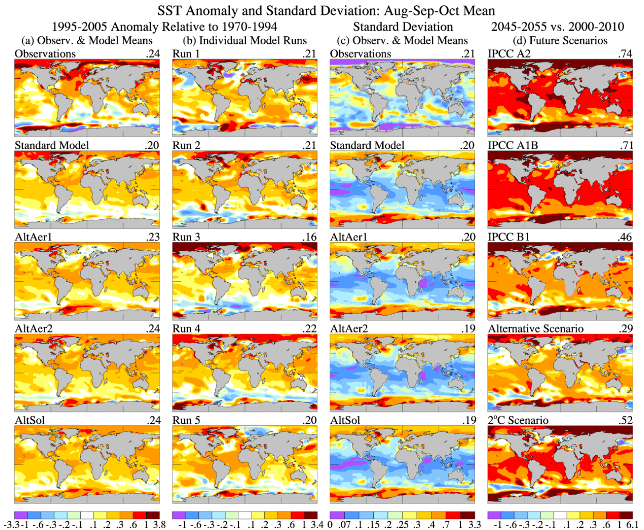
Figure 6. (a) 1995-2005 Aug-Oct SST anomalies relative to 1970-1994 base period, the top map for observations and next four for several ‘all forcing’ ensembles, (b) 1995-2005 Aug-Oct SST anomalies relative to 1970-1994 for individual ensemble members of the standard ‘all forcings’ simulation, (c) standard deviations among successive decadal means relative to immediately preceding 25 years, (d) simulated 2045-2055 Aug-Oct SST anomalies relative to the present (2001-2009 mean).
