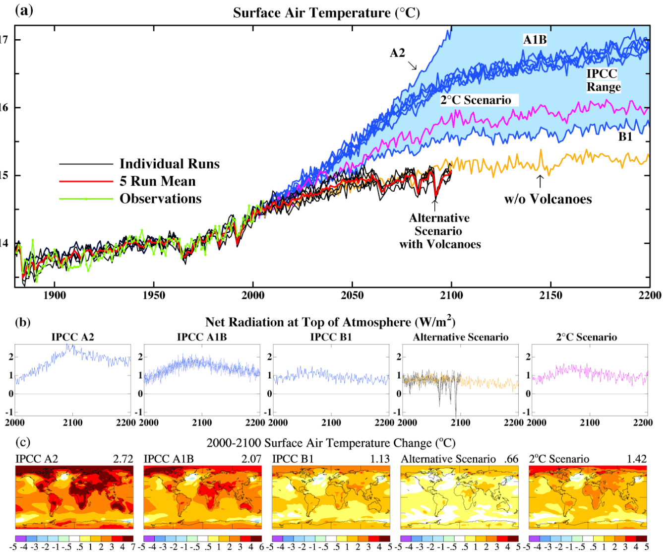
Figure 3. Global mean surface air temperature for several scenarios calculated by our coupled climate model as extensions of the 1880-2003 simulations for “all forcings”. Forcings beyond 2003 for these scenarios are defined in Figure 2. Stratospheric aerosols in 2010-2100 are the same as in 1910-2000 for the case including future volcanoes. Tropospheric aerosols are unchanging in the 21 st century.
