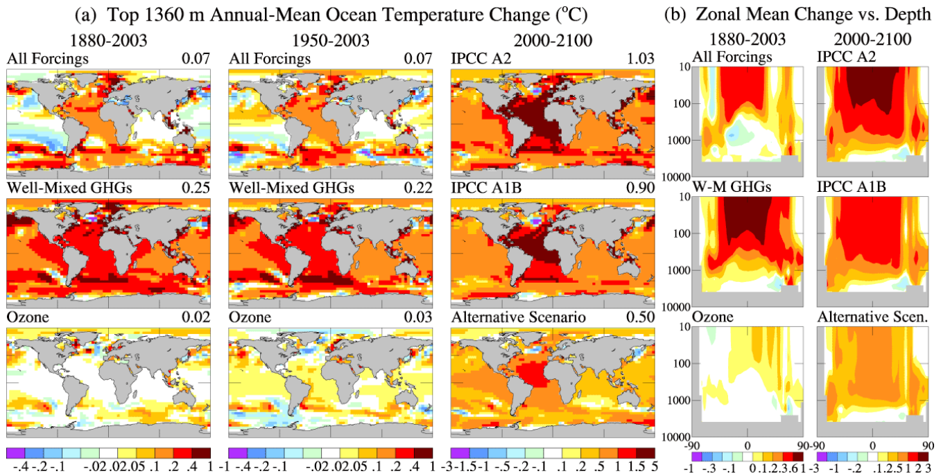
Figure 7. (a) Temperature change in the top 10 layers (1360 m) of the ocean for three periods and three forcings, (b) zonal-mean ocean temperature change for these forcings. Positive and negative temperature intervals are symmetric about zero.
