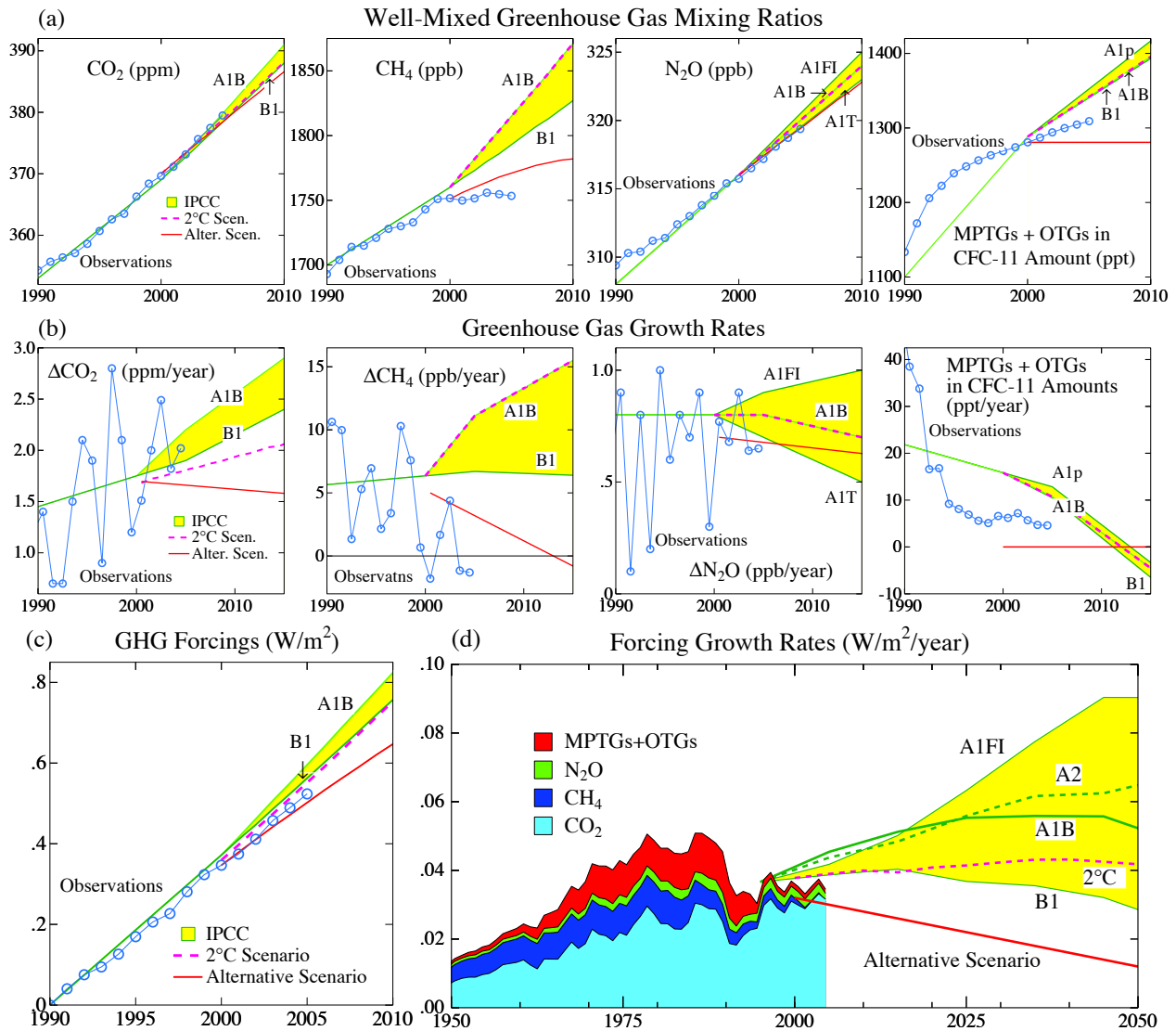
Figure 8. (a) Greenhouse gas amounts, (b) growth rates, and (c) resulting forcings and (d) forcing growth rates for IPCC [2001], “alternative”, and “2°C” scenarios [Hansen et al. , 2000; Hansen and Sato, 2004]. Observations are 5-year running means of data described by Hansen and Sato [2004] and in the text. Data for recent decades are those reported by the NOAA Earth System Research Laboratory, Global Monitoring Division ( www.cmdl.noaa.gov ). MPTGs and OTGs without available observations (4.9% of the MPTG + OTG estimated forcing in 2000) were assumed to follow IPCC scenario A1B, which probably exaggerates their forcing, as all measured MPTGs and OTGs are currently falling below their IPCC scenarios.
