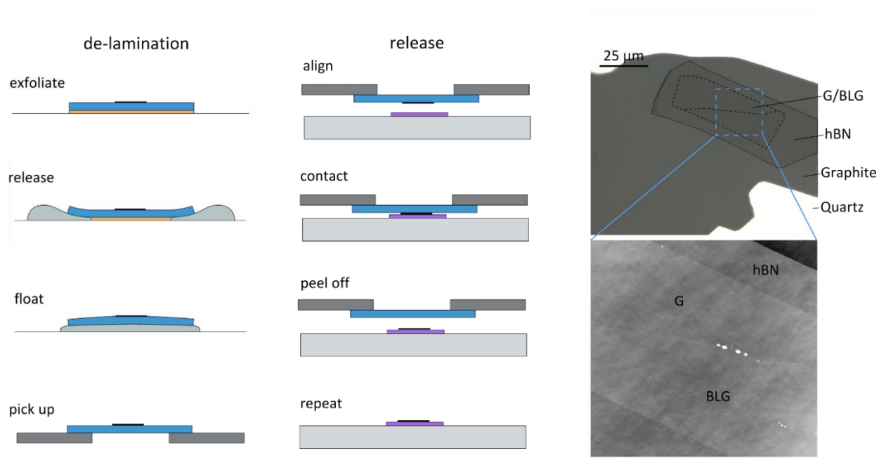
Figure S1. Dry-peel transfer. Left - Different steps of the transfer procedure. Right - Optical micrograph of non-encapsulated graphene/hBN/graphite heterostructure (top); Zoom-in by using AFM in the tapping mode (bottom).
