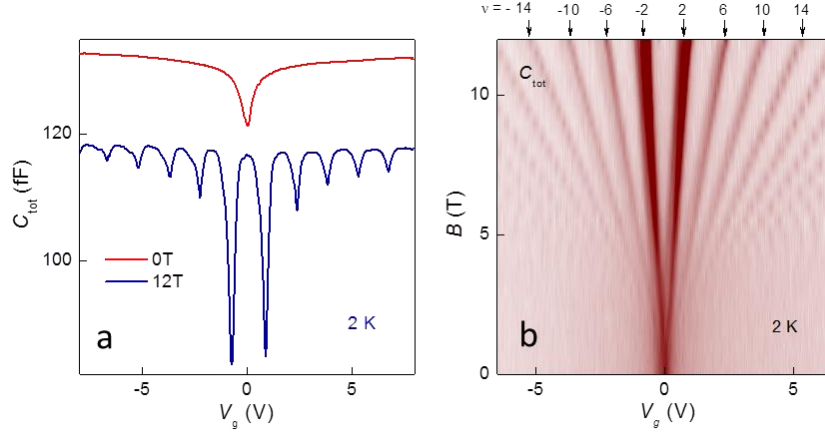
Figure 3. Capacitance spectroscopy of \text{WS}_2/\text{graphene}/\text{hBN}/\text{Au} . (a) C_{\text{tot}} as a function of V_g in zero and quantizing B . For clarity, the 12T curve is offset by 15 fF. (b) Landau fan diagram C_{\text{tot}}(V_g, B) . Scale: wine to white 0.105 to 0.120 pF.
