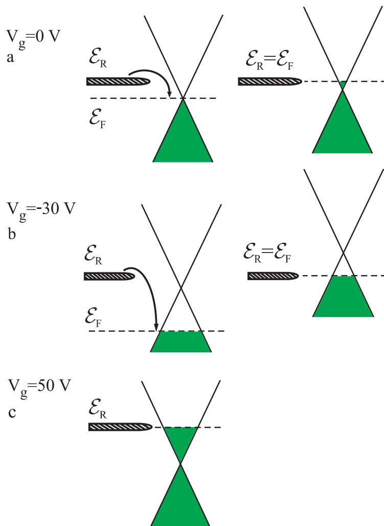
Figure 6: Energy diagram of graphene bands during electrochemical doping. The Fermi level \mathcal{E}_F and redox level \mathcal{E}_R are shown before (left) and after (right) doping by toluene. Three regimes are shown: (a) \mathcal{E}_R > \mathcal{E}_F , V_g = 0 ; (b) \mathcal{E}_R \gg \mathcal{E}_F , negative V_g ; (c) \mathcal{E}_R < \mathcal{E}_F , positive V_g .
