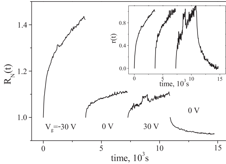
Figure 4: Time dependence of the (normalised) resistance, R_N , after rapid changes in the gate voltage: from V_g = 0 to -30 V, to 0, to +30 V, and back to 0. Inset: data as in main figure but normalised by the full resistance range, r = (R - R_{\min}) / (R_{\max} - R_{\min}) .
