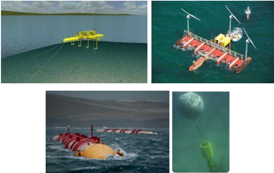
Figure 7: Example WEC devices ( top left ) Bluewater BlueTEC floating platform and ( top right ) Poseidon Floating Power platform. ( bottom left ) Pelamis Wave Power P2 wave energy converter and ( bottom right ) Carnegie Wave Energy CETO wave energy converter
