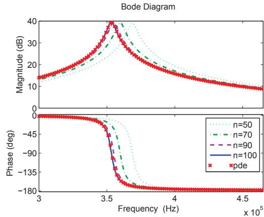
Fig. 3. Discretized Bode diagrams for G_{pu}(s) for different values of n
