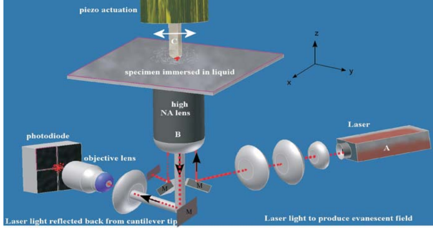
Fig. 1. Simplified schematic of the TDFM together with SEW system (adopted from [26]).
