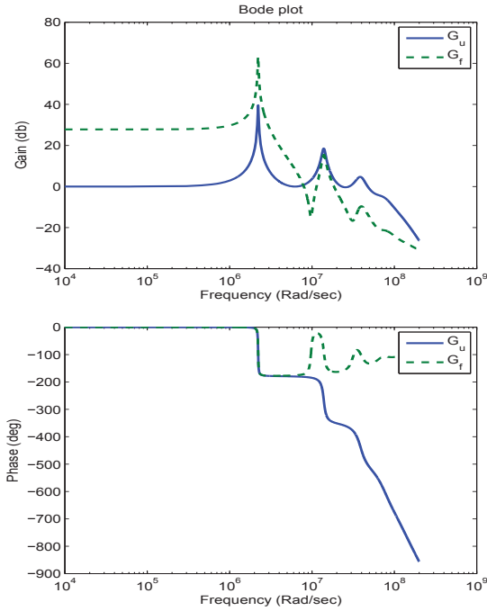
Fig. 4. Magnitude and Phase Plot of G_{pu}(s) = C_p(sI - A_p)B_p and G_{pf}(s) = C_p(sI - A_p)D_p
