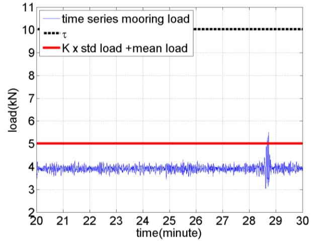
Fig. 9 Example of a 10 minute dataset showing a large mooring load compared to the adjacent mooring loads, but with not sufficient overall amplitude to be considered as an extreme mooring load
