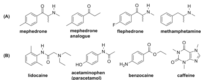
Fig. 1. Structures of mephedrone, and related chemical analogues (A) and cutting agents (B).
