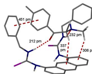
Fig. 3. DFT fully optimized structure of probe 2 complexed with mephedrone highlighting the array of intermolecular interactions ( \pi - \pi , CH \cdots \pi , NH \cdots N and NH \cdots OC).
