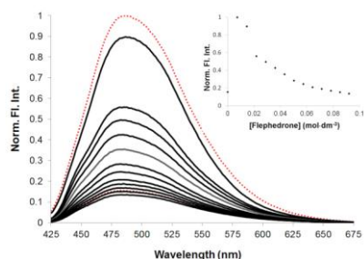
Fig. 4. Normalized fluorescent titration of probe 2 with neat flephedrone (red lines indicate probe 2 only and the first aliquot) Insert: Plot of flephedrone concentration and the quenching of fluorescence intensity at 485 nm (acetone, 5 \times 10^{-6} mol·dm ^{-3} , \lambda_{\text{ex}} = 410 nm).
