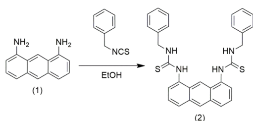
Scheme 1. Synthesis of molecular probe 2 .
