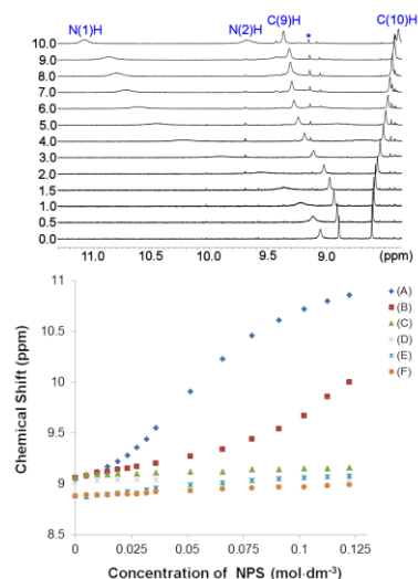
Fig. 2. (Top) Partial 1 H-NMR spectra showing titration of probe 2 with the addition of mephedrone; (*) is suspected cycloaddition product. (Bottom) Chemical shift changes observed for the NH(1) signal, upon the addition of (A) mephedrone, (B) flephedrone, (C) methamphetamine, (D) 1-( p -tolyl)propan-1-one (mephedrone analogue), (E) and (F) compound 3 upon the addition of mephedrone and flephedrone, respectively.
