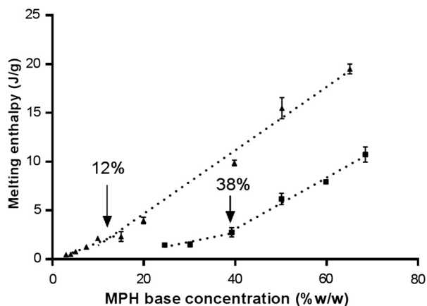
Fig. 4. The melting enthalpy curve for physical mixtures of varying proportions of MPH-base with EuE (■) and EuRS (▲) ( n = 3 , error bars represent the range).
