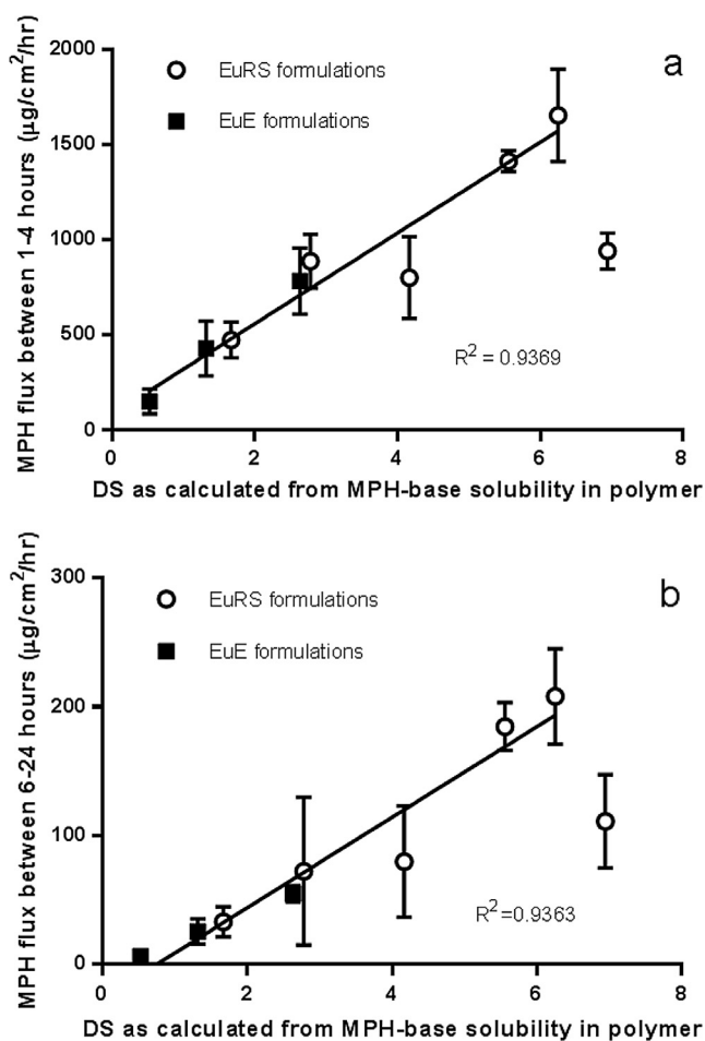
Fig. 8. MPH flux between (a) 1 and 4 h and (b) 6 and 24 h plotted against the degree of saturation as calculated from the MPH-base solubility within EuRS (○) or EuE (■) for formulations of varied MPH-base content containing 3% PG, 6% EuRS or EuE, 30% IPA and DME ( n = 5-6 \pm SD ).
