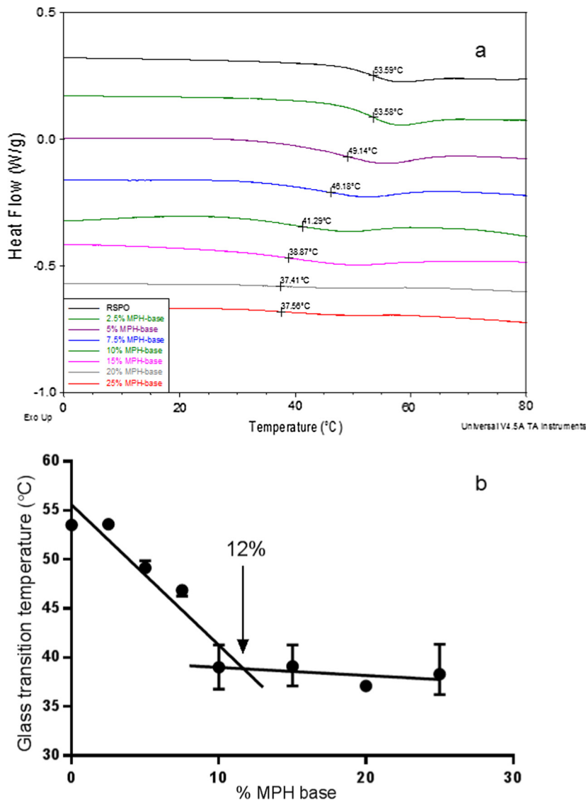
Fig. 5. (a) Representative DSC curves for solvent cast film solid dispersions of varying proportions of MPH-base with EuRS and (b) the glass transition temperatures for these films plotted against drug loading ( n = 3 , error bars represent the range).
